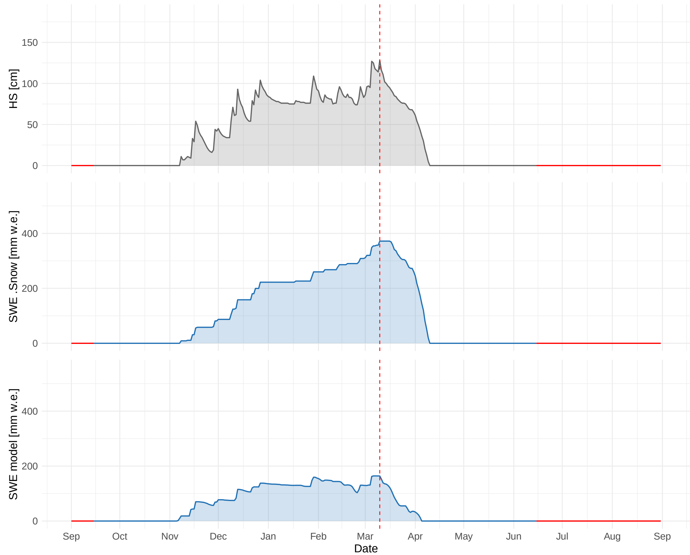
HSD_CH_BLA (1538 m a.s.l.) – 2019 to 2020
