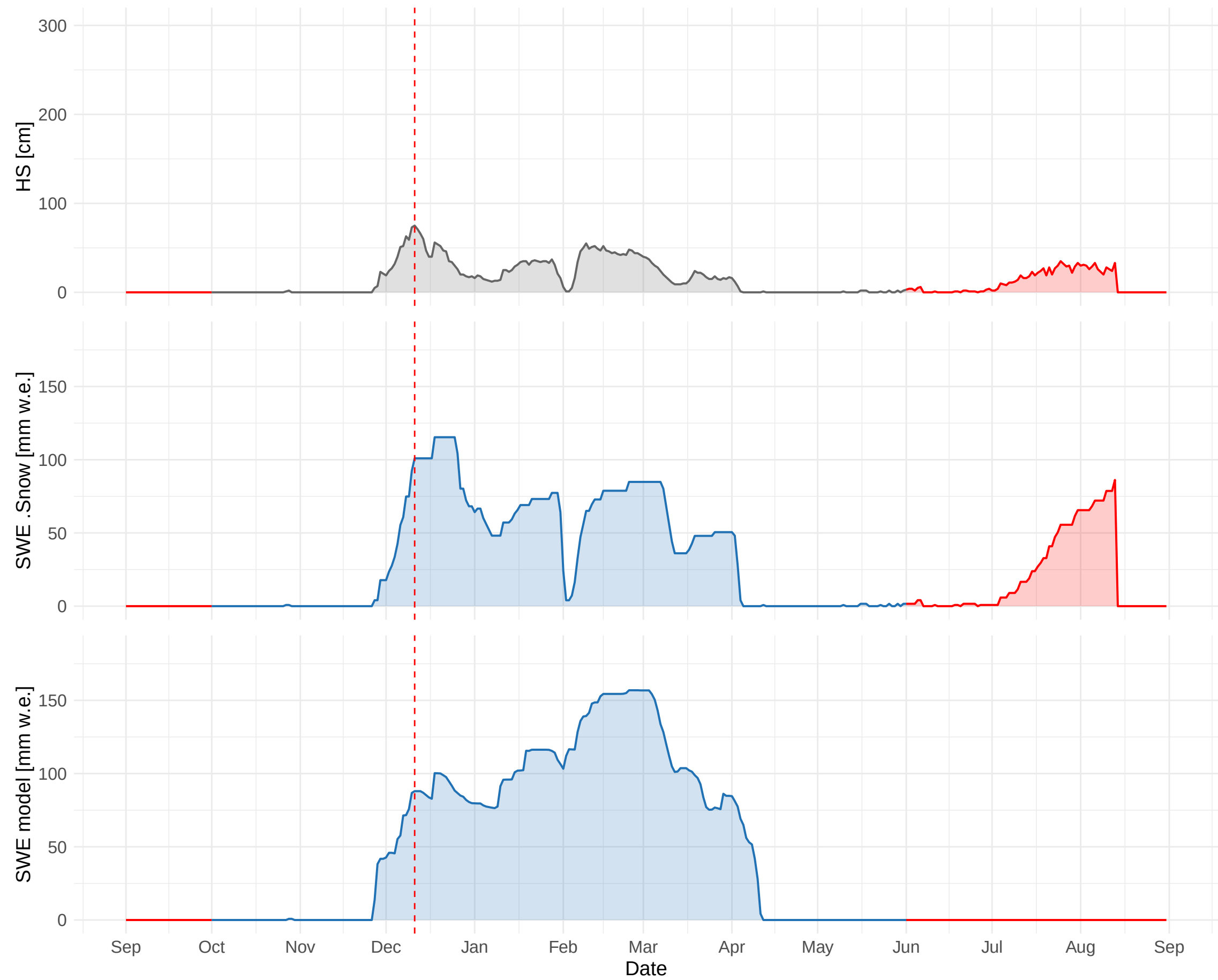
HSD_CH_CDF (1017 m a.s.l.) – 2012 to 2013
