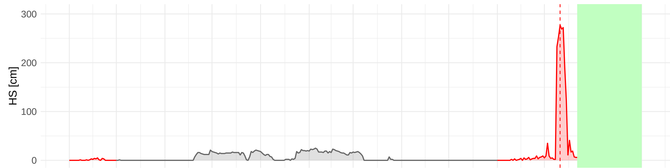
HSD_CH_CDF (1017 m a.s.l.) – 2013 to 2014
