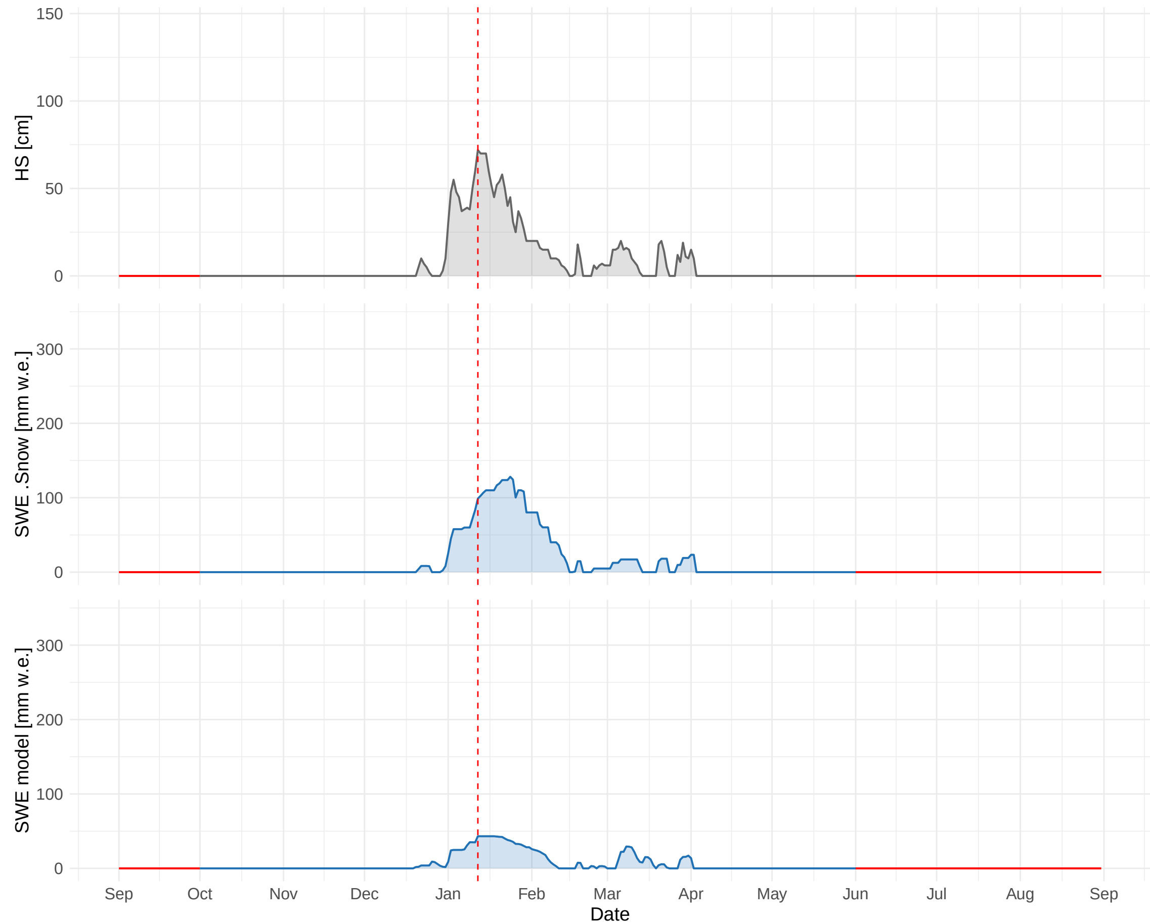
HSD_CH_CDF_MAN (1017 m a.s.l.) – 1994 to 1995
