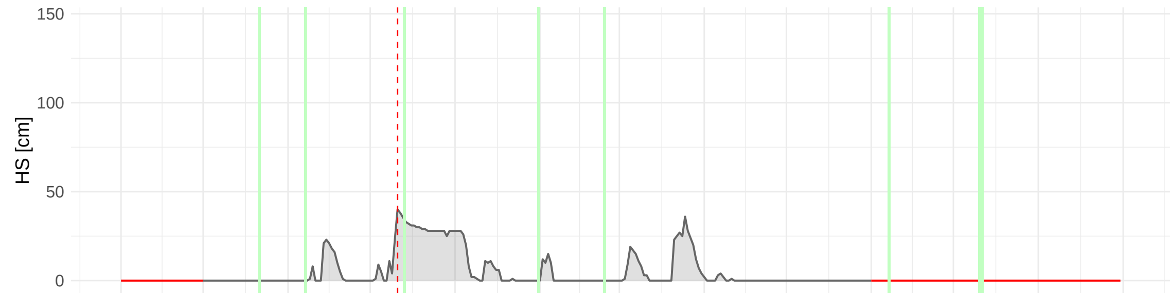
HSD_CH_CDF_MAN (1017 m a.s.l.) – 2007 to 2008
