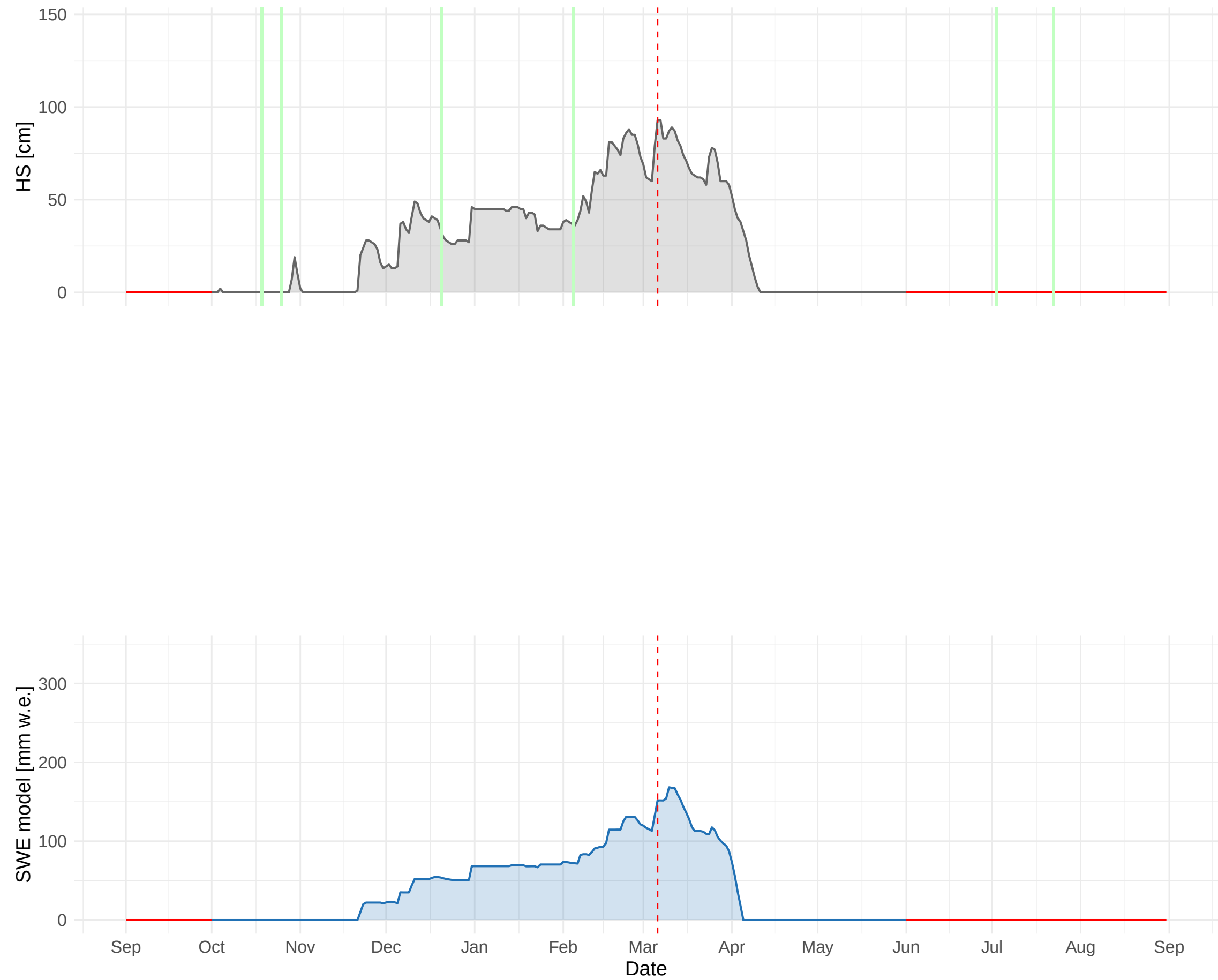
HSD_CH_CDF_MAN (1017 m a.s.l.) – 2008 to 2009
