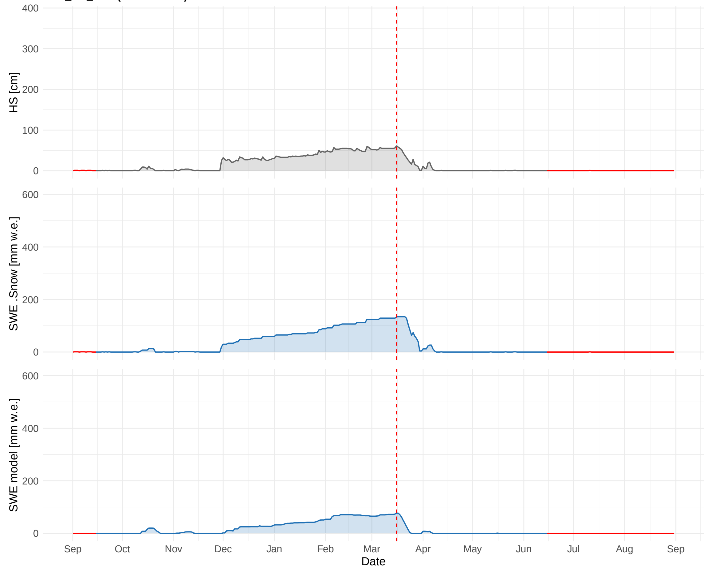
HSD_CH_DAV (1594 m a.s.l.) – 2009 to 2010
