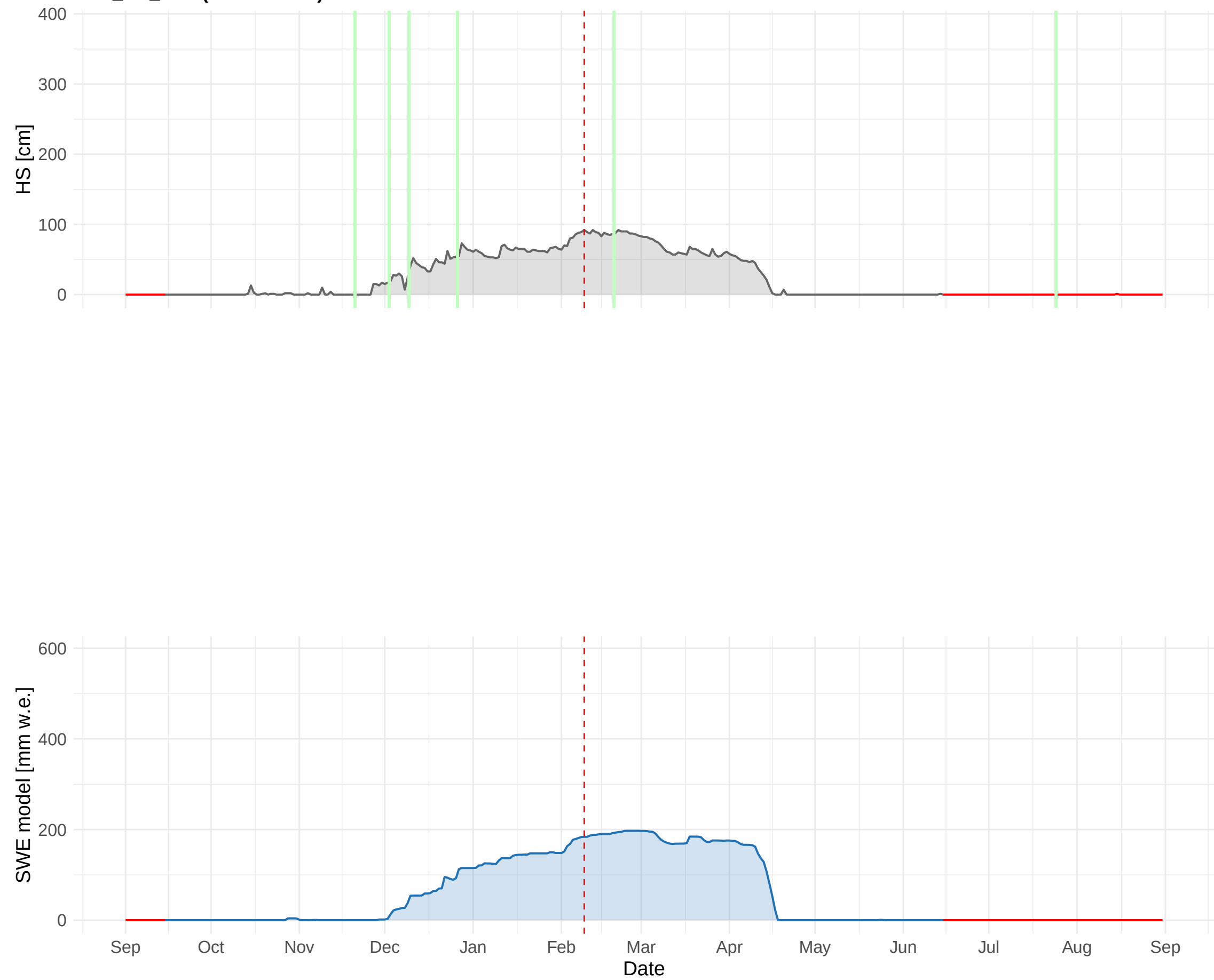
HSD_CH_DAV (1594 m a.s.l.) – 2012 to 2013
