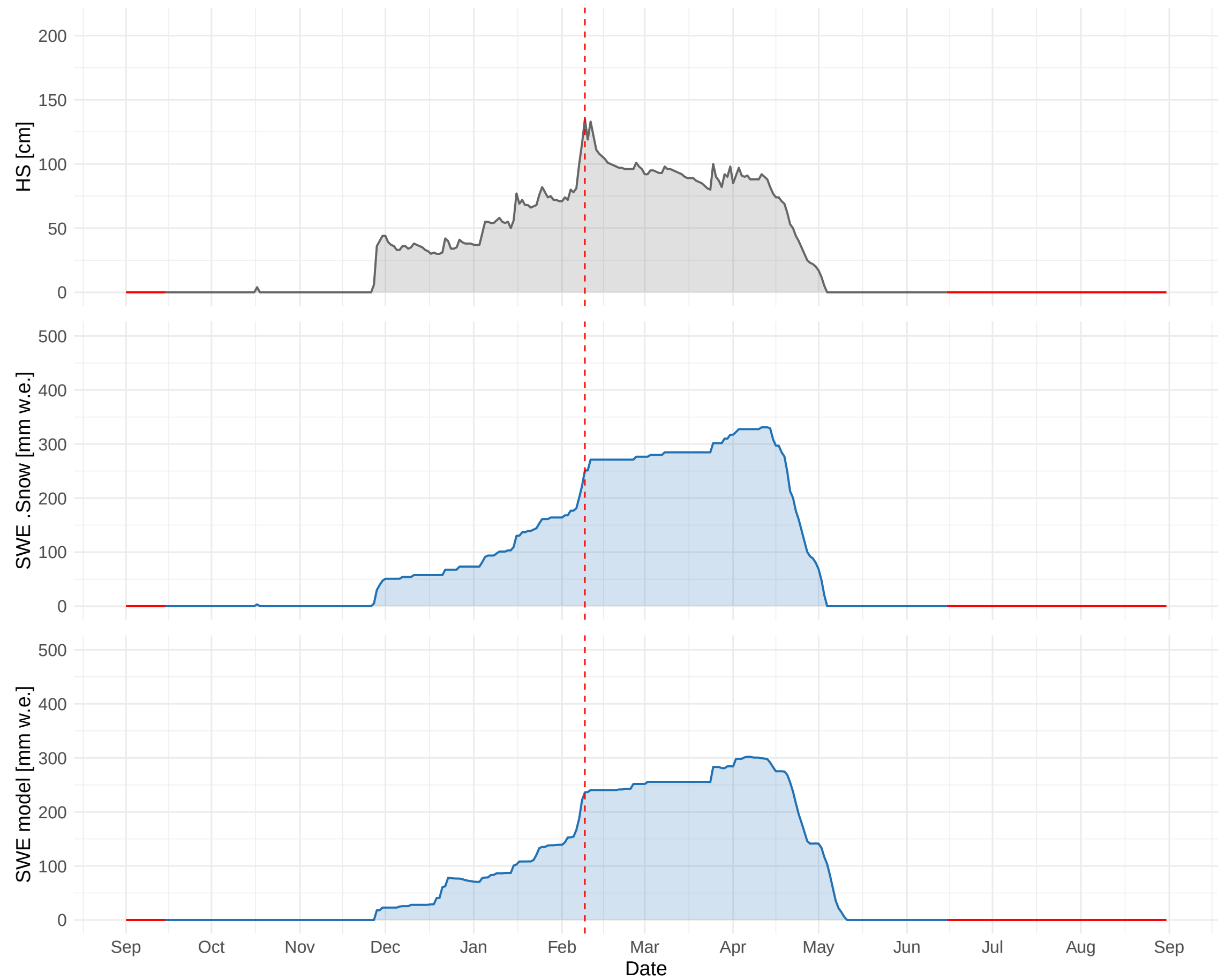
HSD_CH_DAV_MAN (1594 m a.s.l.) – 1983 to 1984
