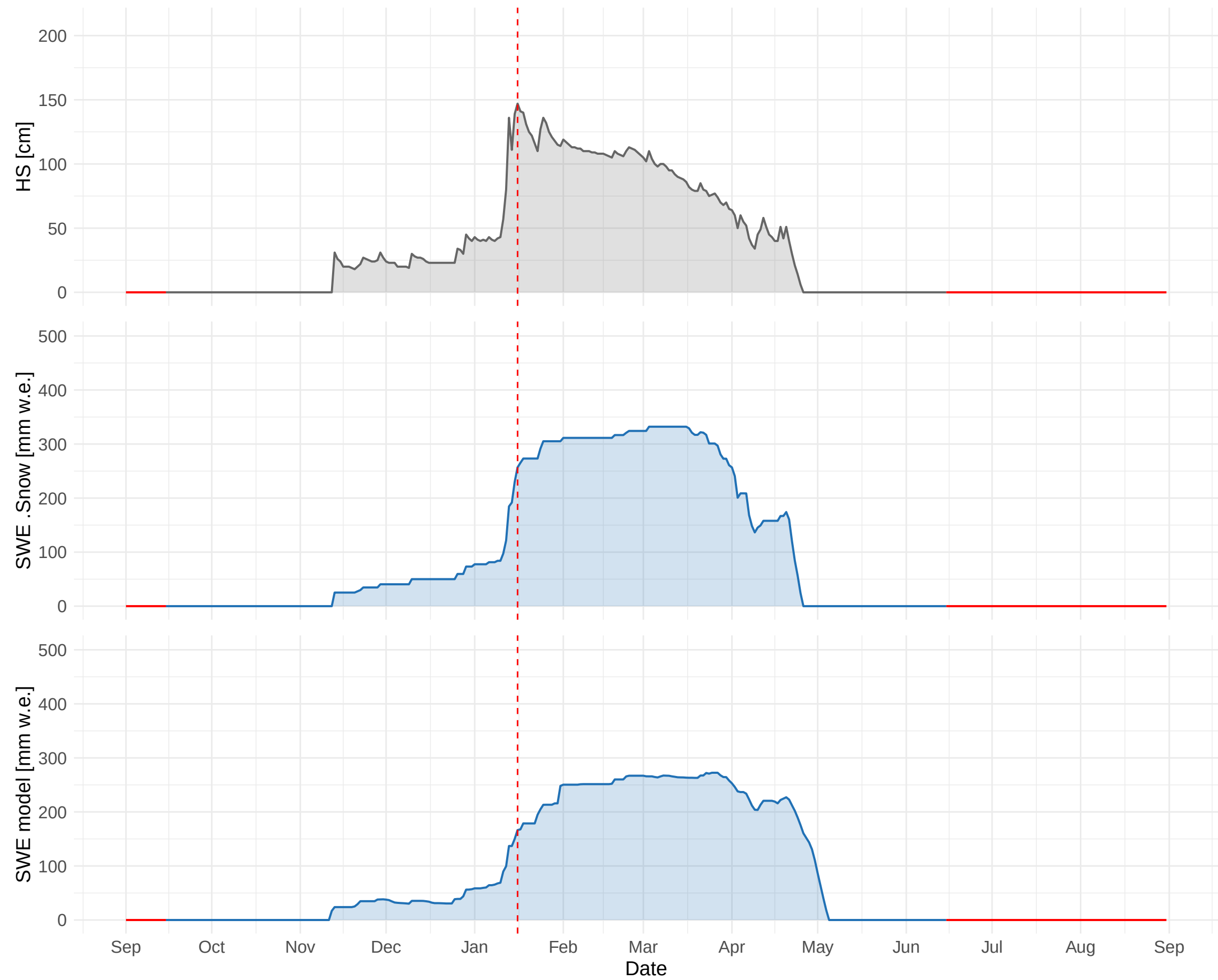
HSD_CH_DAV_MAN (1594 m a.s.l.) – 1985 to 1986
