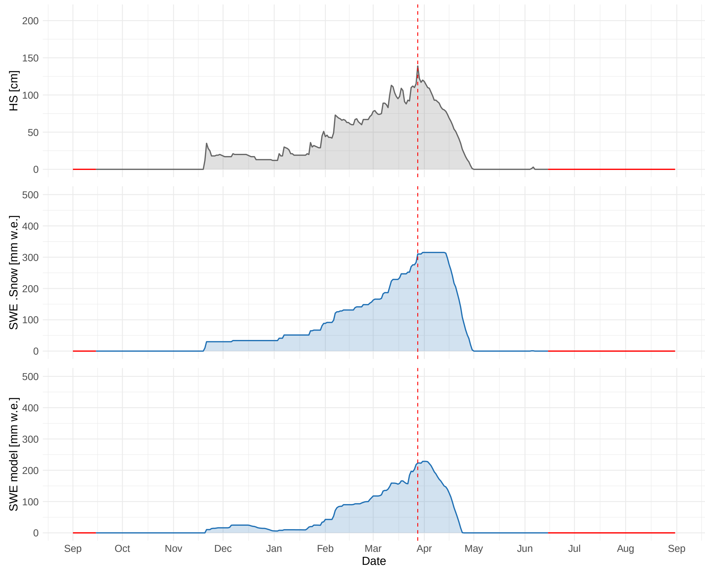
HSD_CH_DAV_MAN (1594 m a.s.l.) – 1987 to 1988
