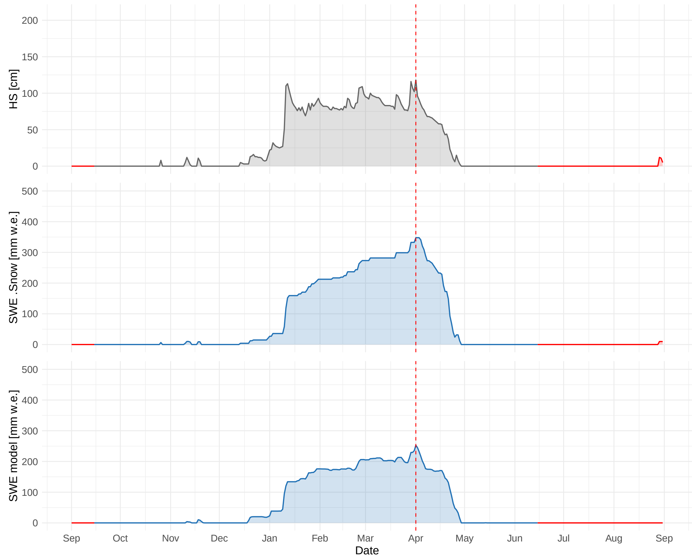
HSD_CH_DAV_MAN (1594 m a.s.l.) – 1994 to 1995
