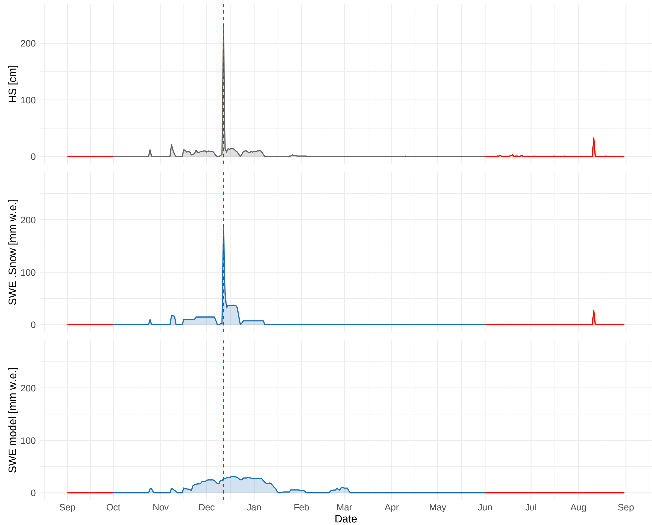
HSD_CH_DIS (1197 m a.s.l.) – 2010 to 2011
