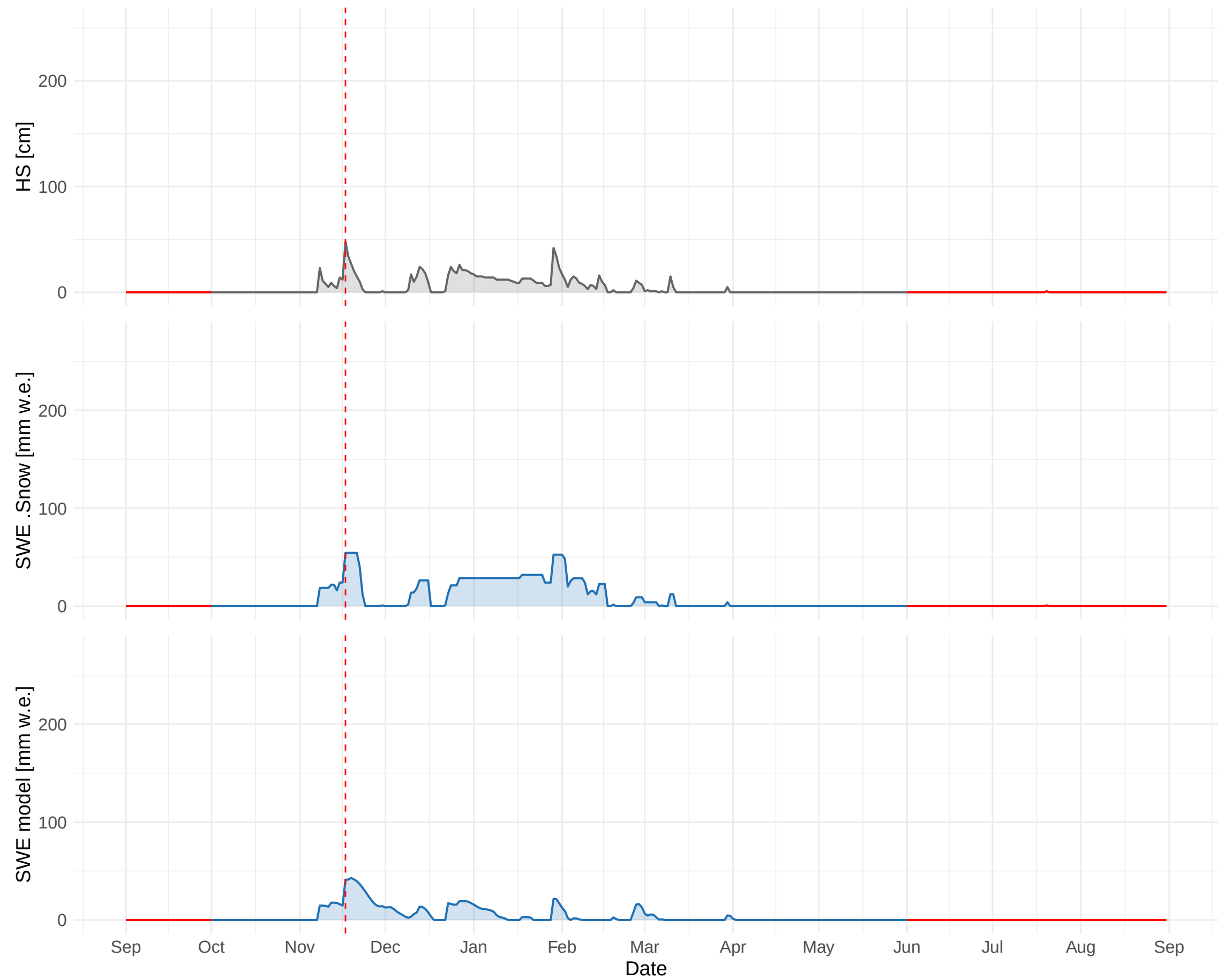
HSD_CH_DIS (1197 m a.s.l.) – 2019 to 2020
