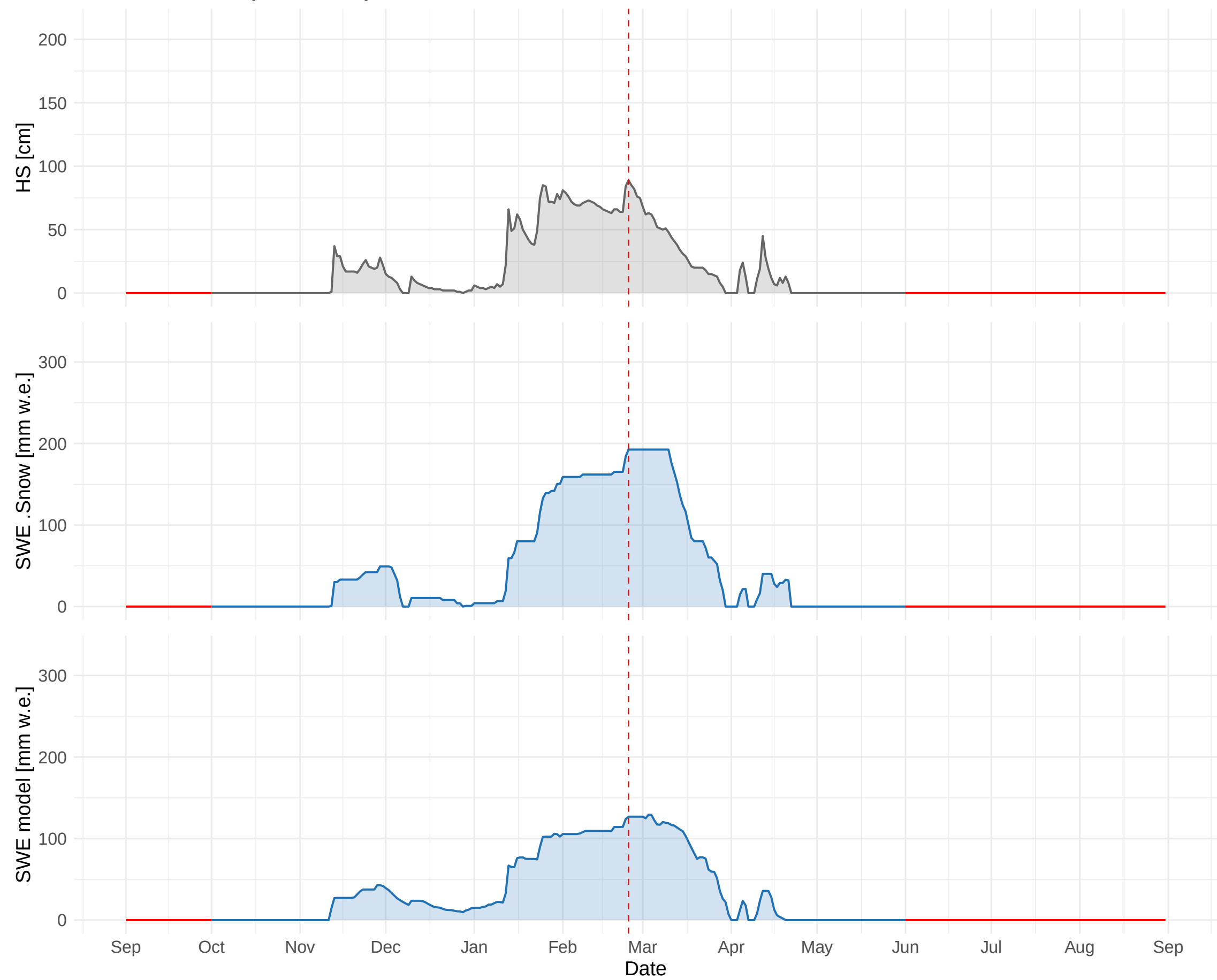
HSD_CH_DIS_MAN (1197 m a.s.l.) – 1985 to 1986
