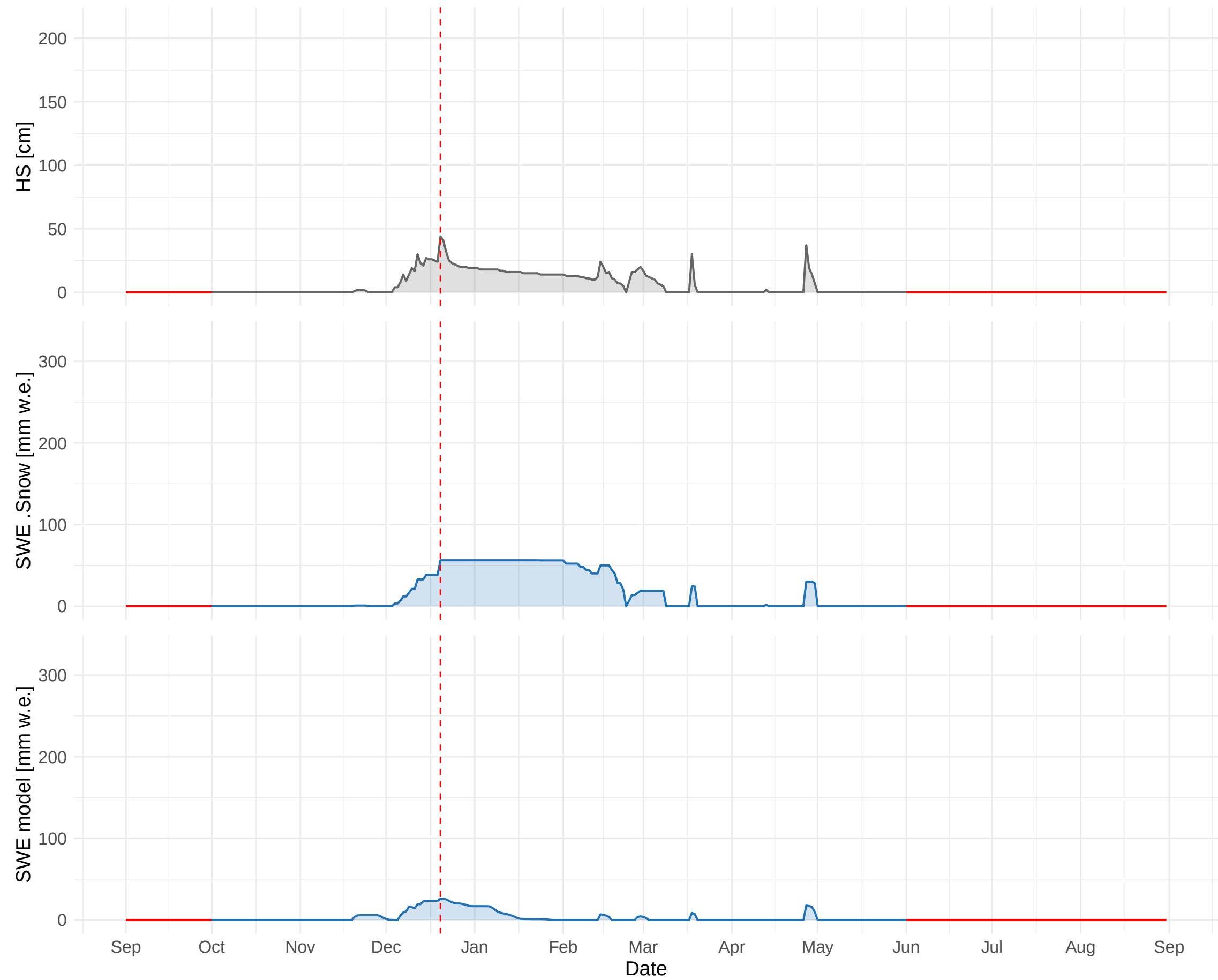
HSD_CH_DIS_MAN (1197 m a.s.l.) – 1988 to 1989
