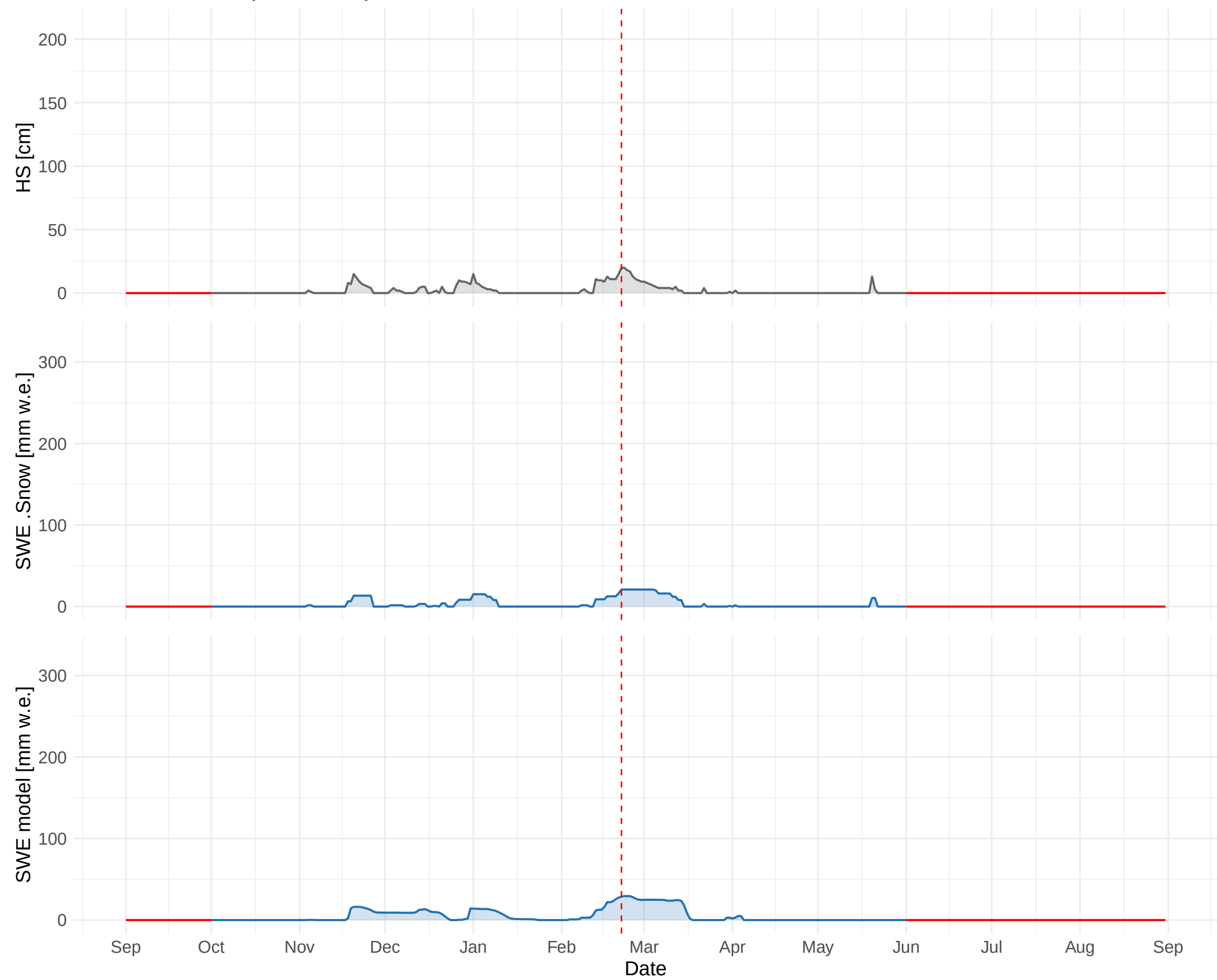
HSD_CH_DIS_MAN (1197 m a.s.l.) – 1995 to 1996
