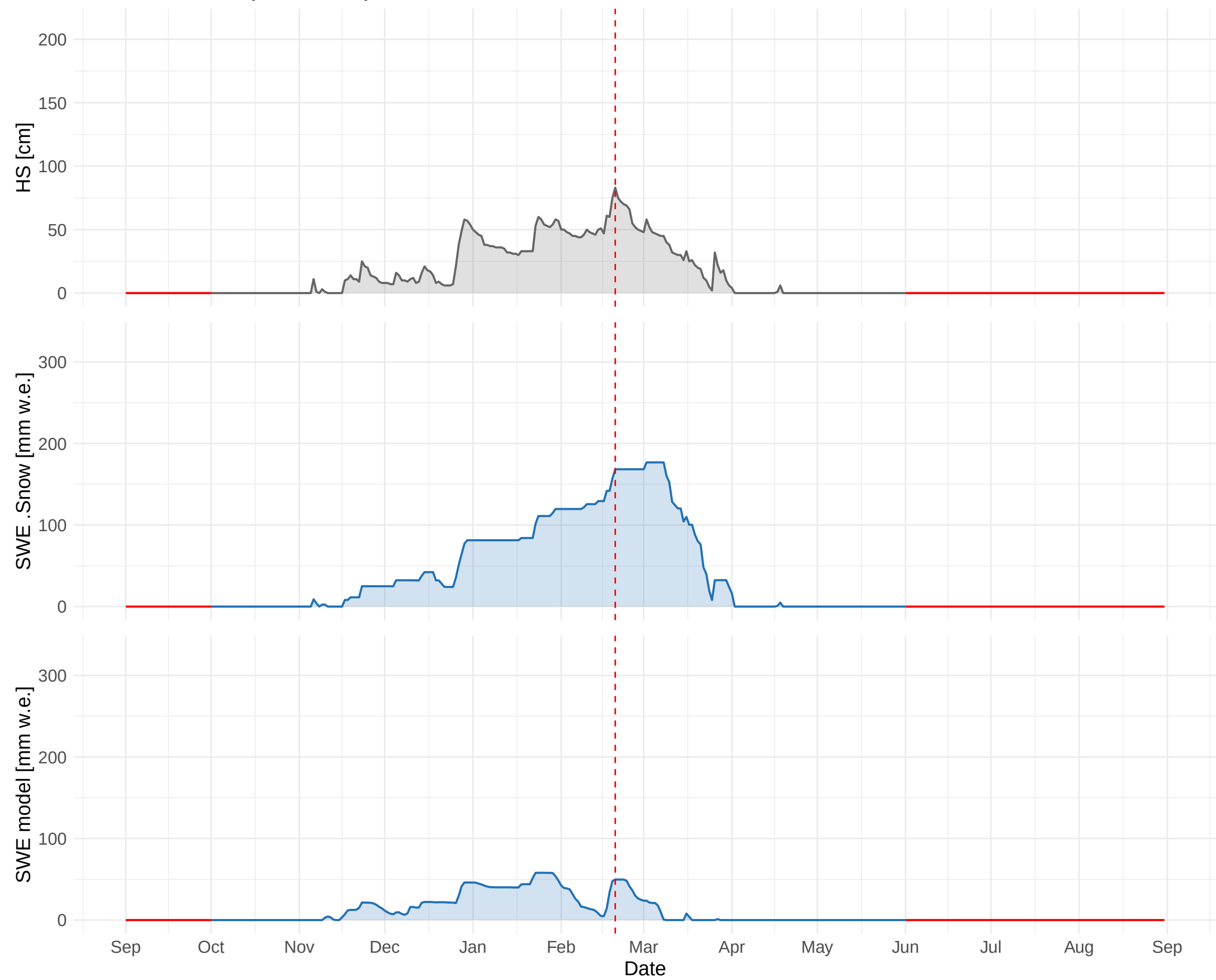
HSD_CH_DIS_MAN (1197 m a.s.l.) – 1999 to 2000
