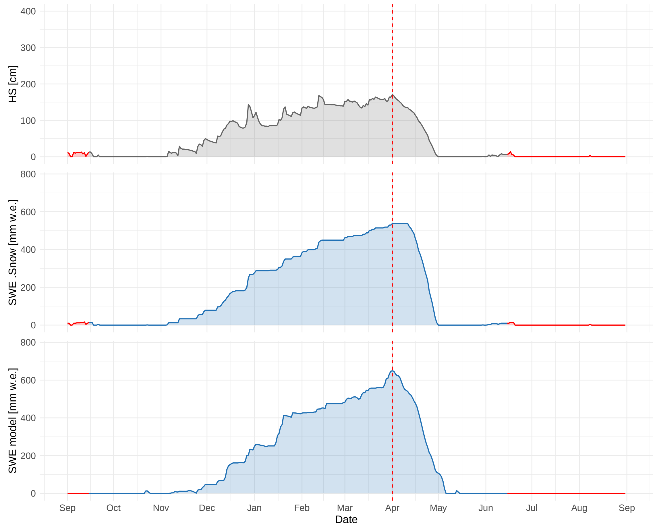
HSD_CH_DOL (1669 m a.s.l.) – 2017 to 2018
