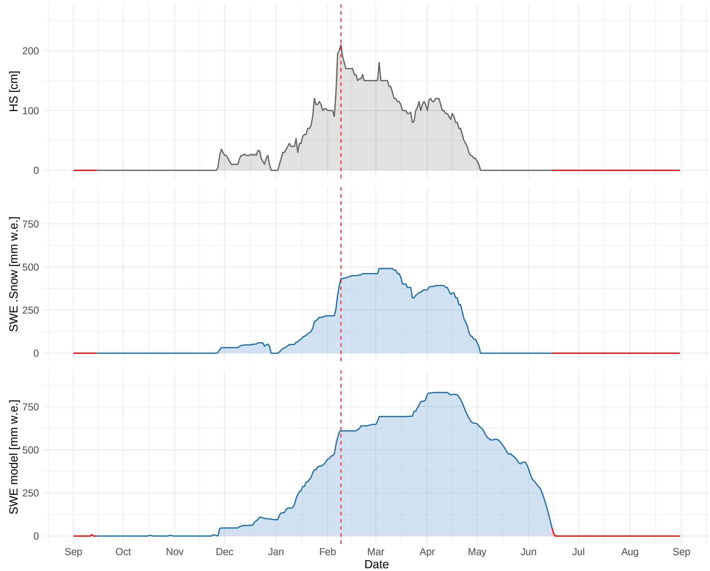
HSD_CH_DOL_MAN (1669 m a.s.l.) – 1983 to 1984
