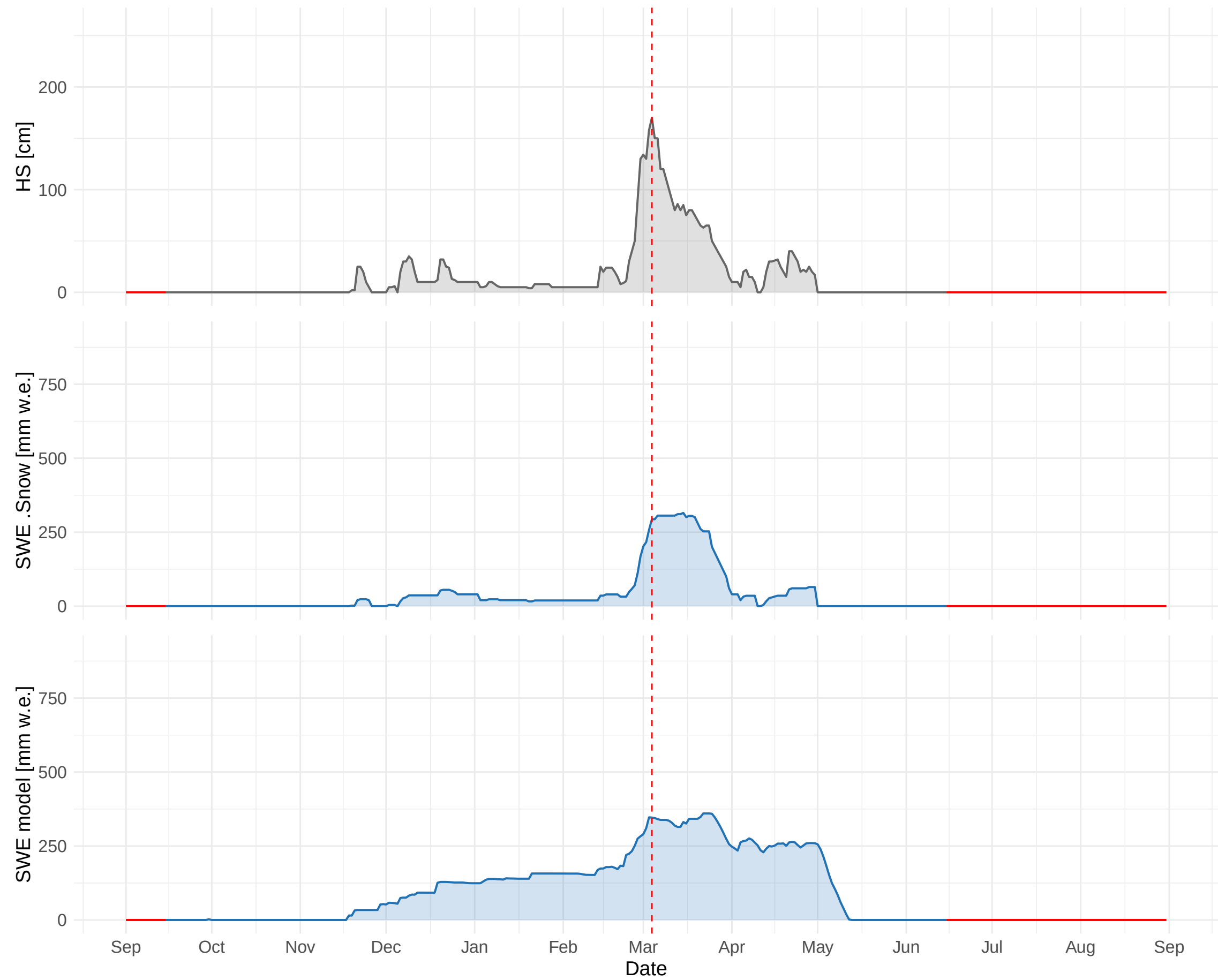
HSD_CH_DOL_MAN (1669 m a.s.l.) – 1988 to 1989
