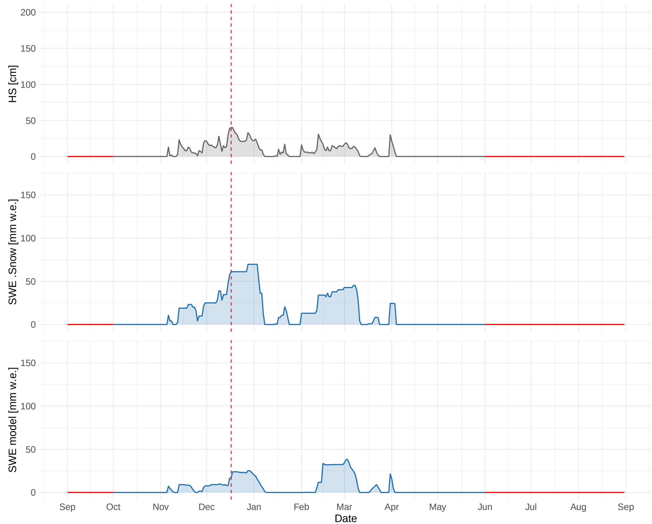
HSD_CH_ENG (1035 m a.s.l.) – 2017 to 2018
