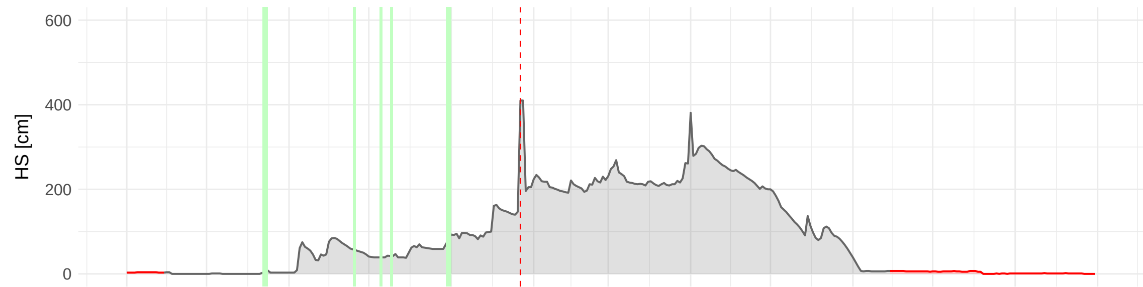
HSD_CH_GRH (1980 m a.s.l.) – 2014 to 2015
