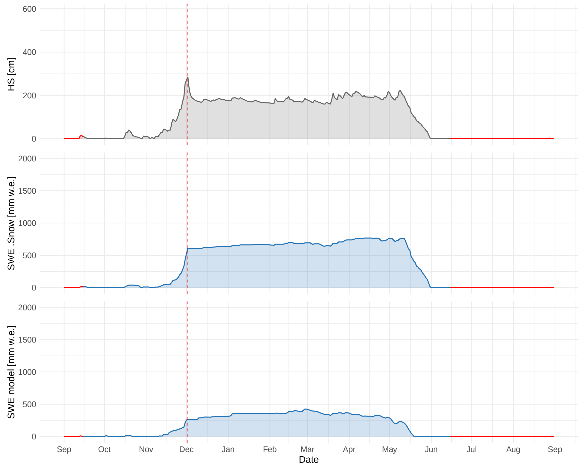
HSD_CH_GRH_MAN (1980 m a.s.l.) – 1996 to 1997
