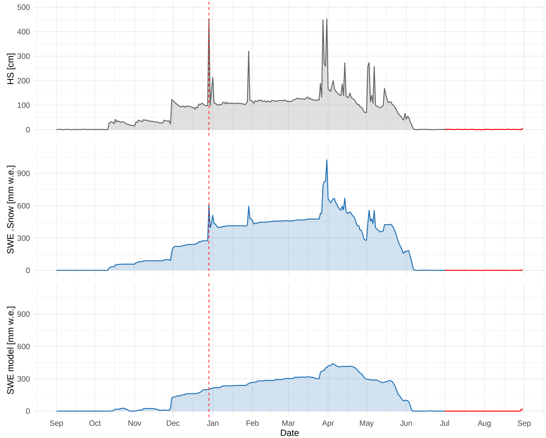
HSD_CH_GUE (2286 m a.s.l.) – 2009 to 2010
