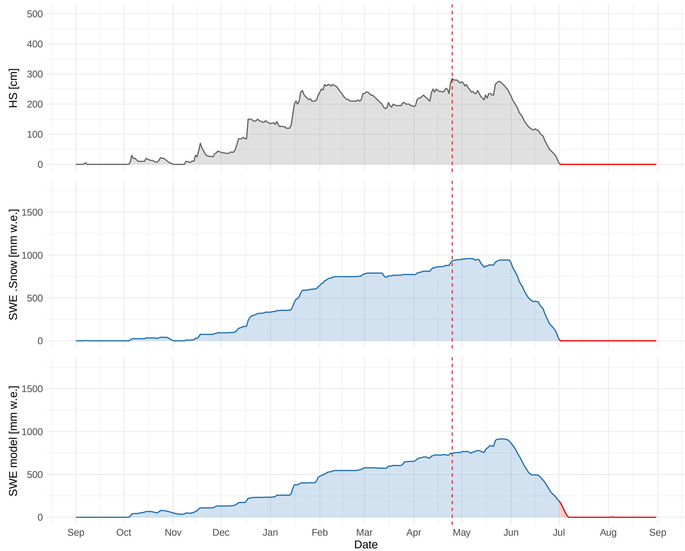
HSD_CH_GUE_MAN (2286 m a.s.l.) – 1982 to 1983
