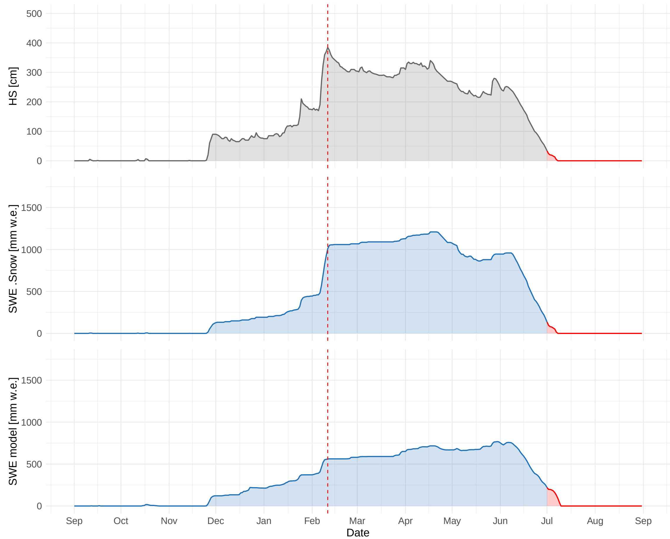
HSD_CH_GUE_MAN (2286 m a.s.l.) – 1983 to 1984
