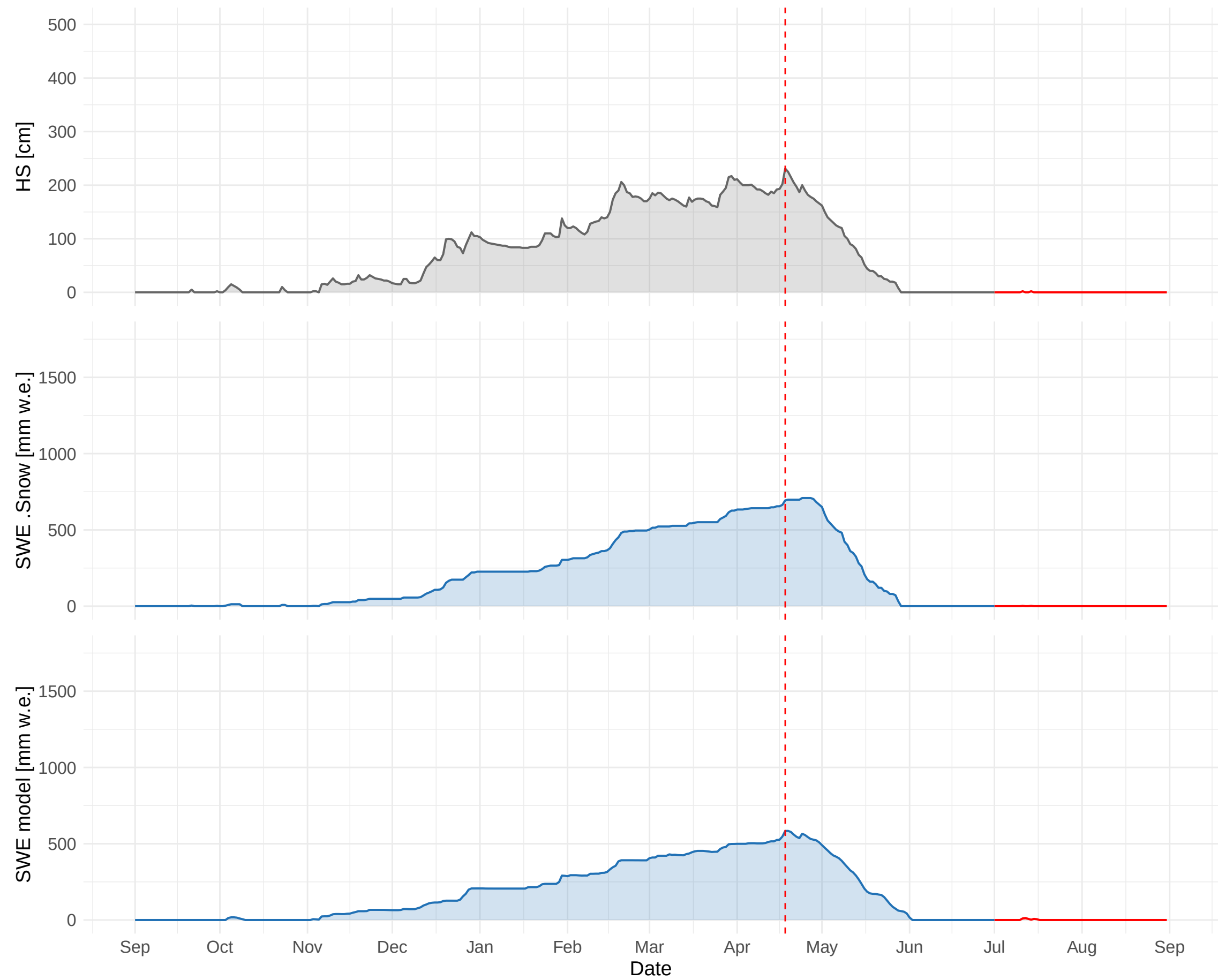
HSD_CH_GUE_MAN (2286 m a.s.l.) – 1999 to 2000
