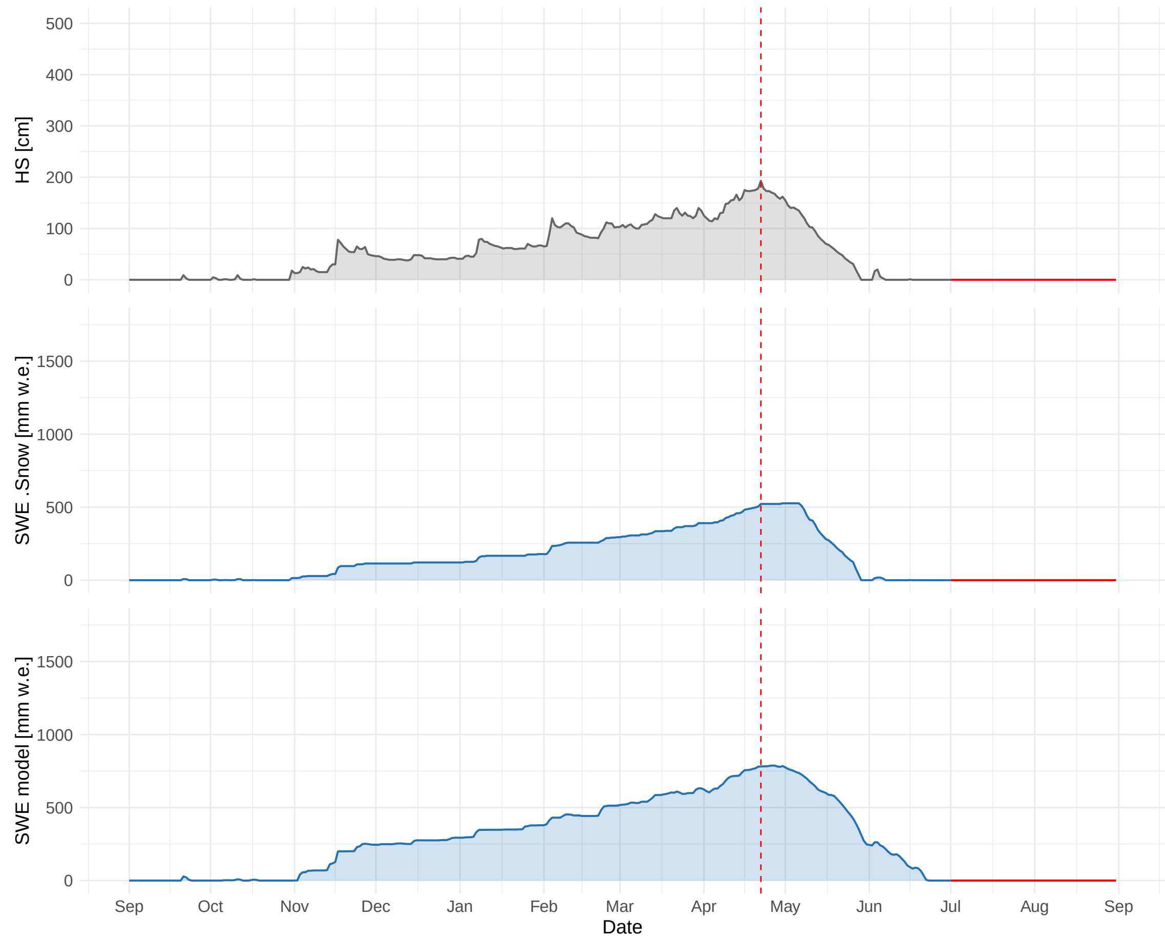
HSD_CH_GUE_MAN (2286 m a.s.l.) – 2000 to 2001
