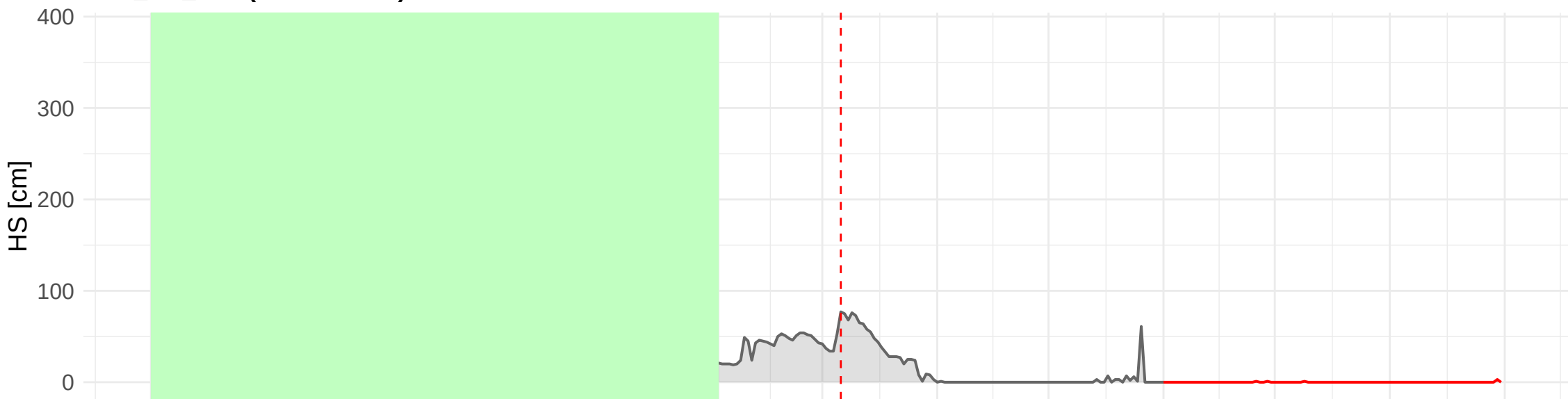
HSD_CH_PLF (1042 m a.s.l.) – 2008 to 2009
