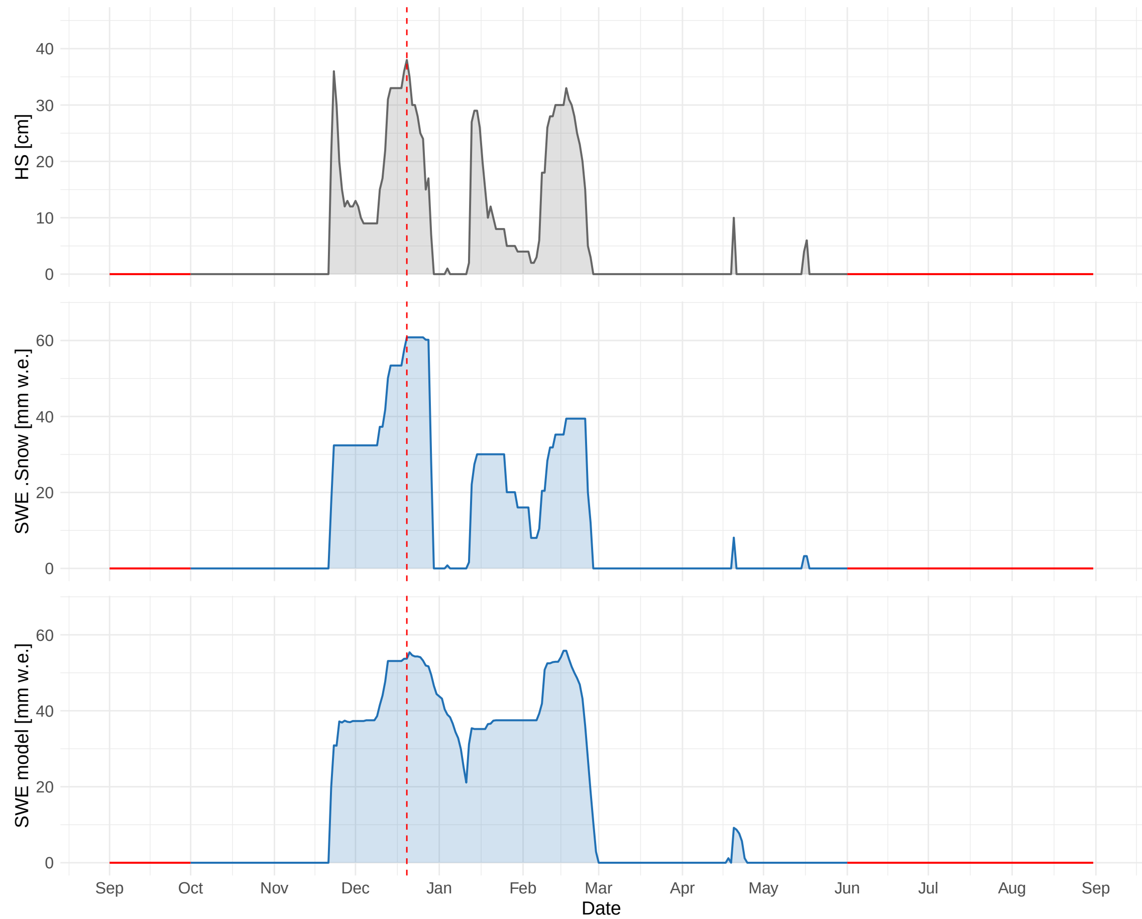
HSD_CH_PLF_MAN (1042 m a.s.l.) – 1990 to 1991
