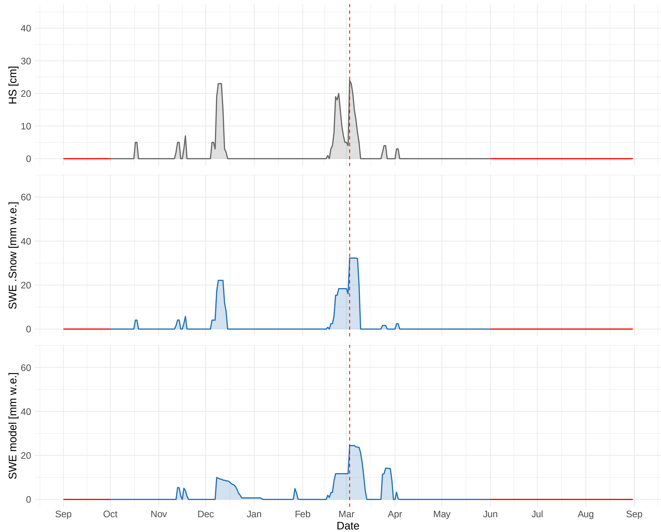
HSD_CH_PLF_MAN (1042 m a.s.l.) – 1992 to 1993
