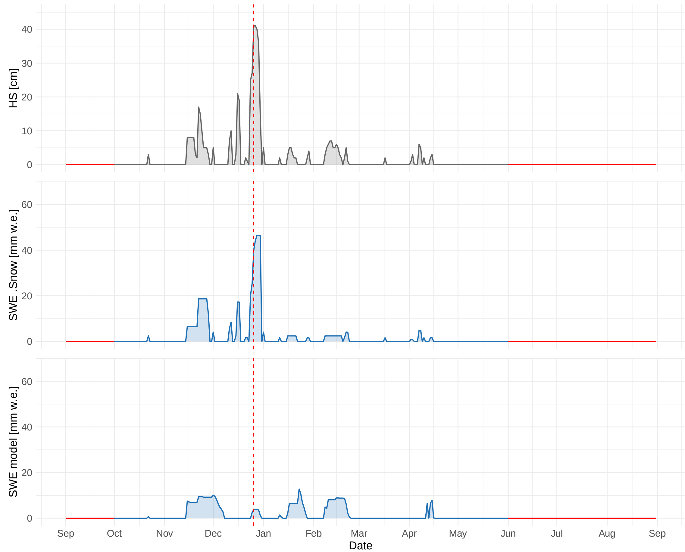
HSD_CH_PLF_MAN (1042 m a.s.l.) – 1993 to 1994
