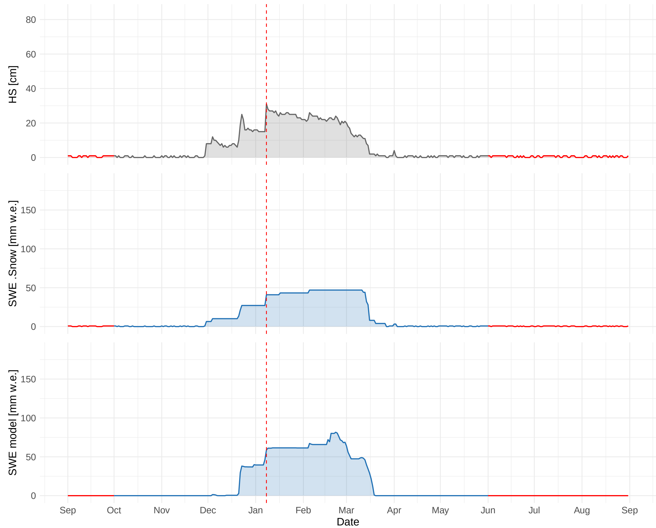
HSD_CH_ROB (1078 m a.s.l.) – 2009 to 2010
