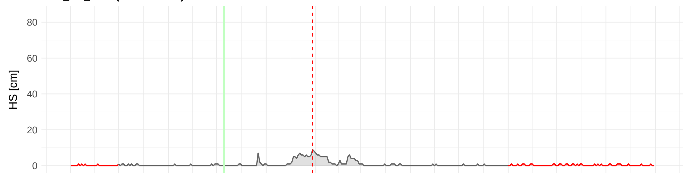
HSD_CH_ROB (1078 m a.s.l.) – 2014 to 2015
