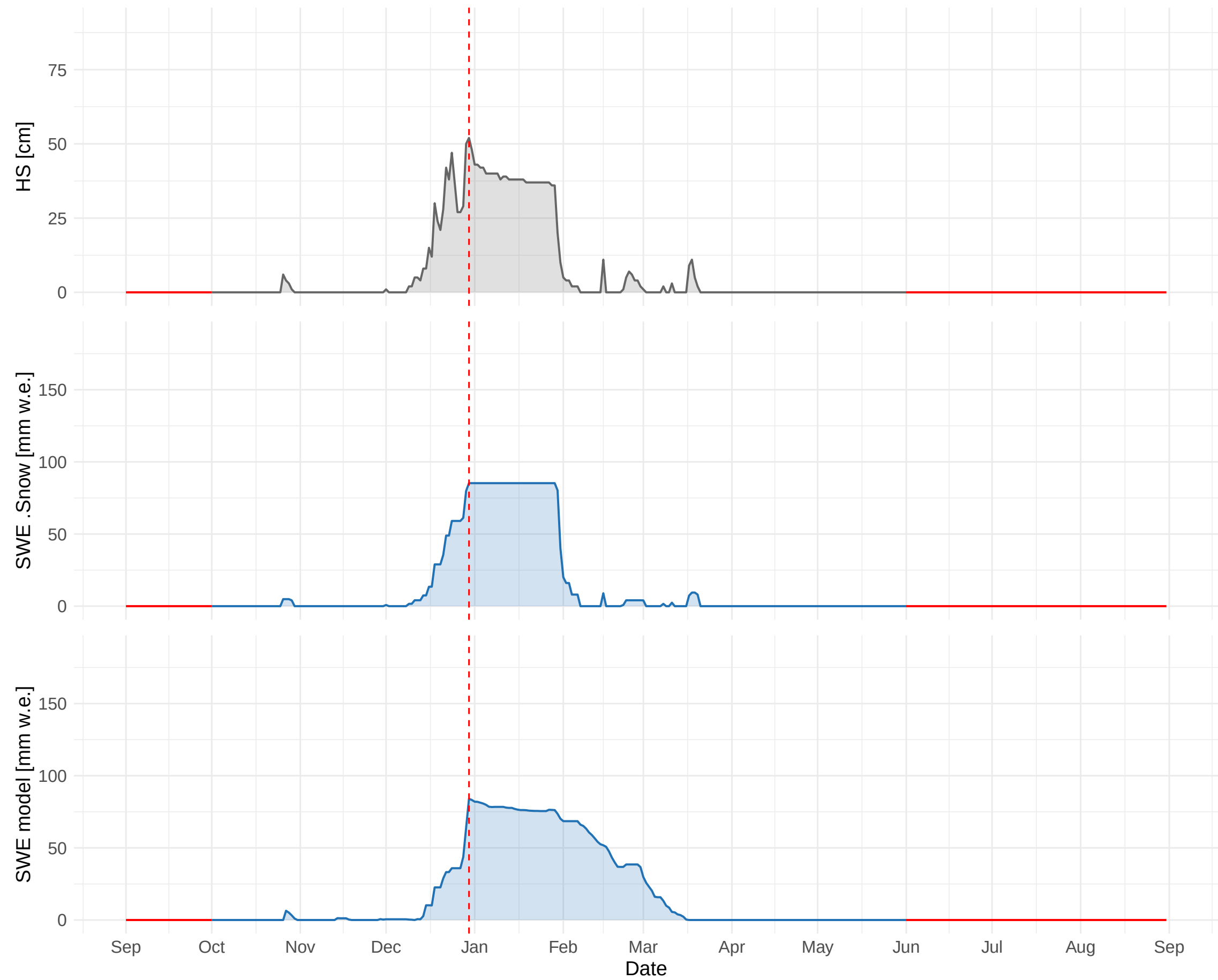
HSD_CH_ROB_MAN (1078 m a.s.l.) – 1981 to 1982
