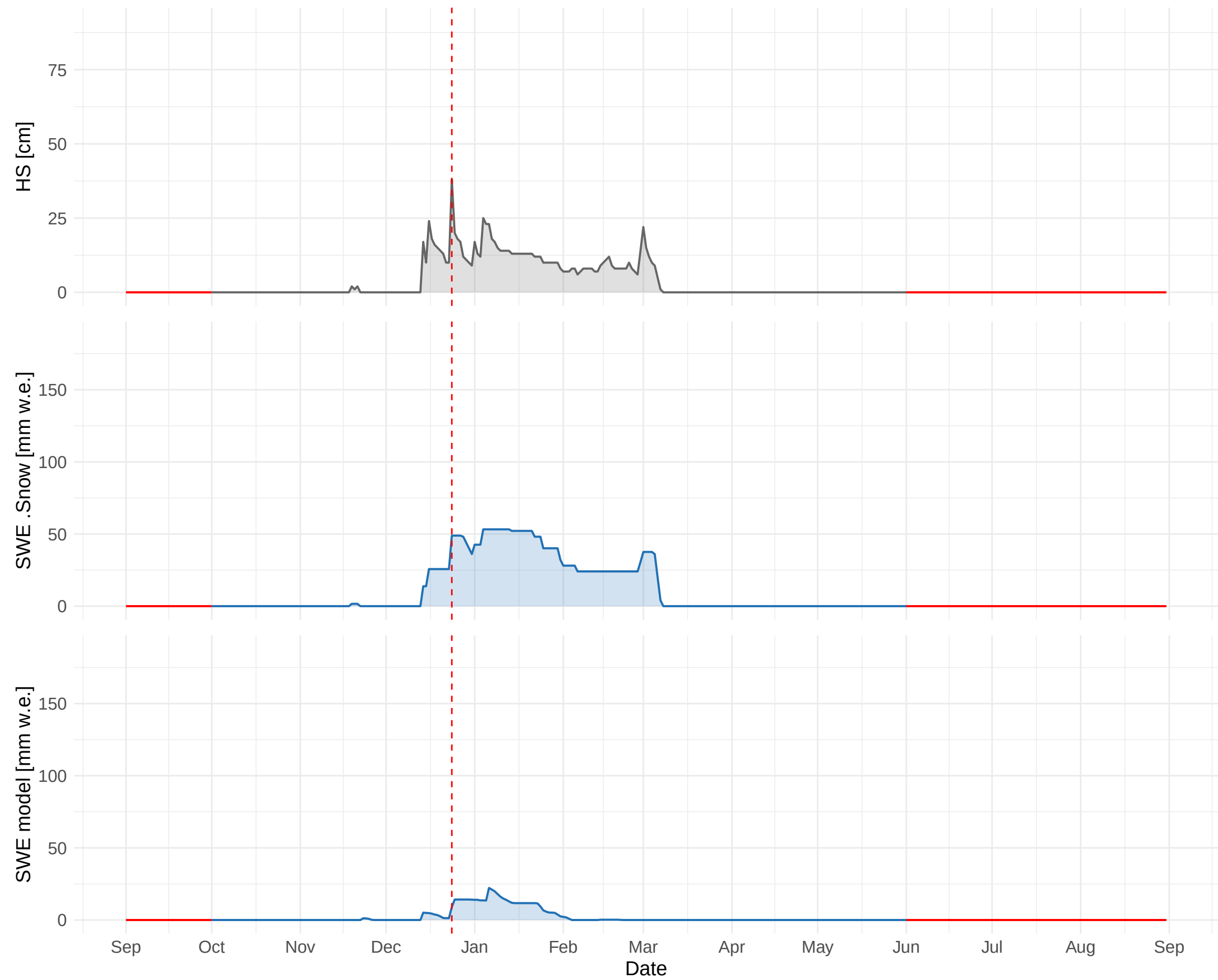
HSD_CH_ROB_MAN (1078 m a.s.l.) – 1993 to 1994
