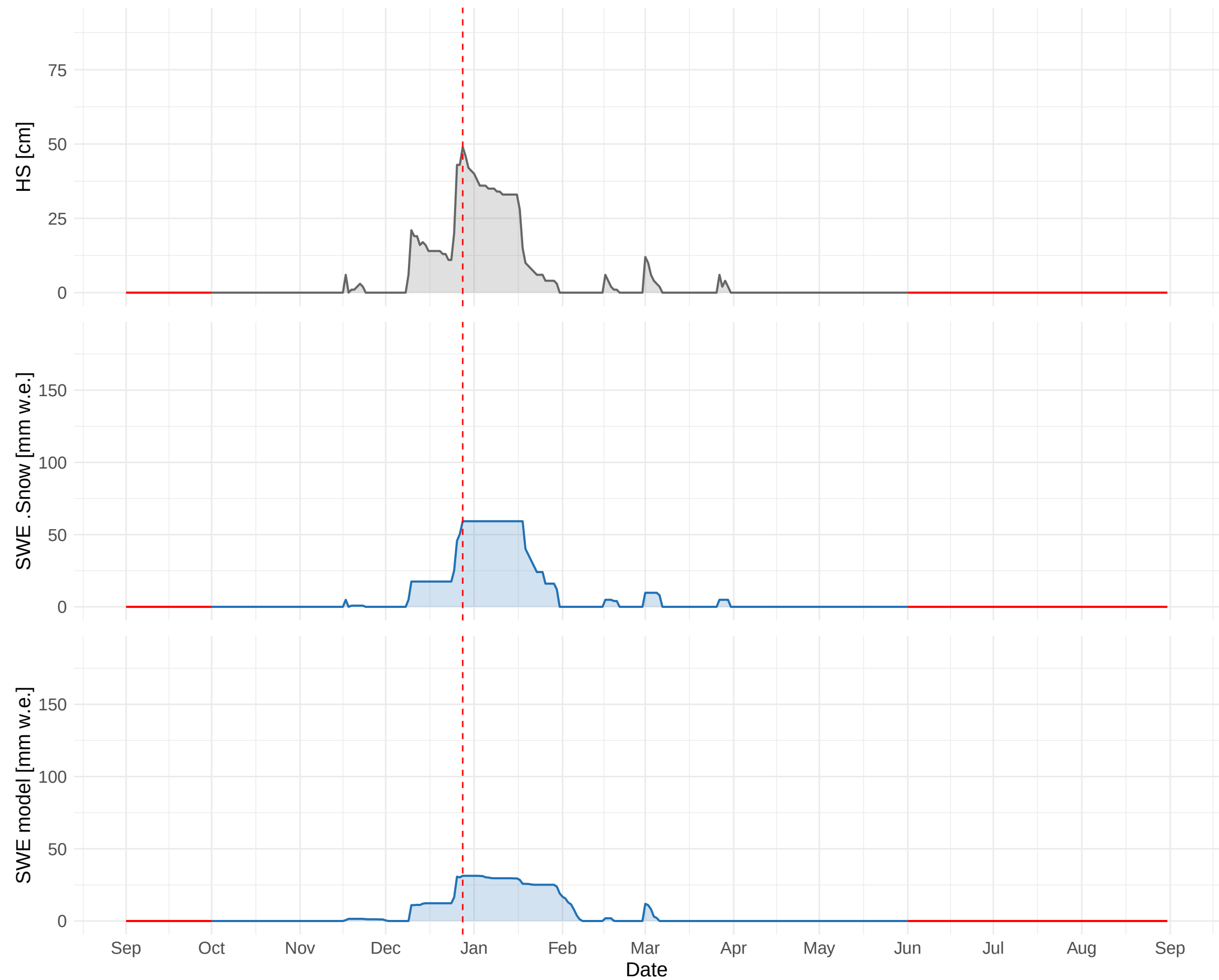
HSD_CH_ROB_MAN (1078 m a.s.l.) – 1999 to 2000
