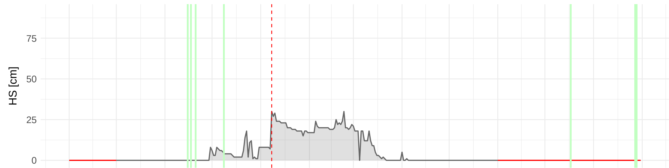
HSD_CH_ROB_MAN (1078 m a.s.l.) – 2009 to 2010
