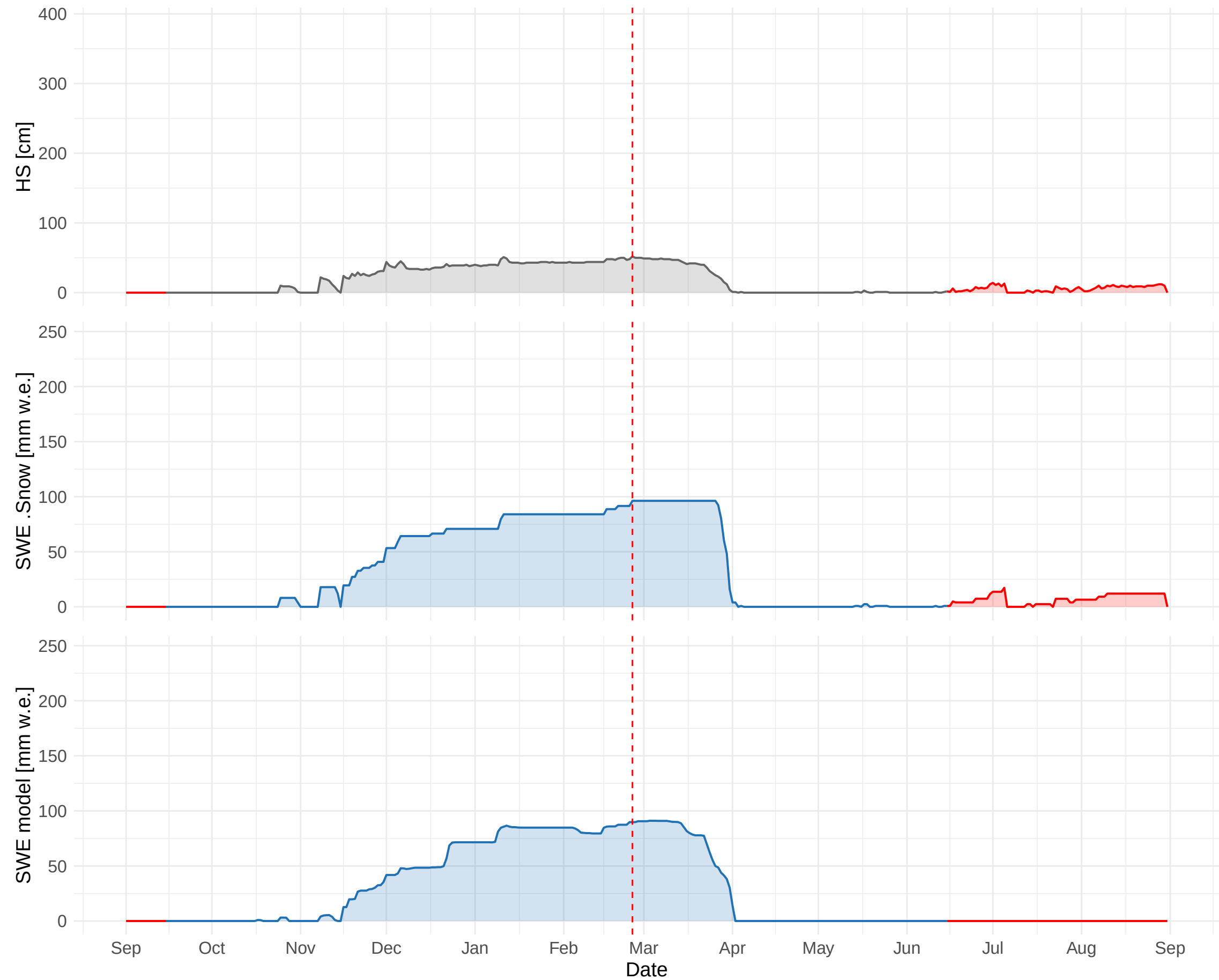
HSD_CH_SAM (1708 m a.s.l.) – 2010 to 2011
