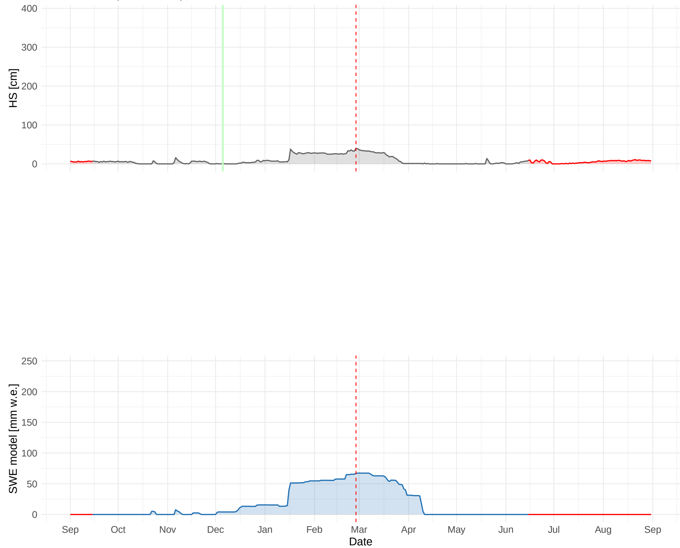
HSD_CH_SAM (1708 m a.s.l.) – 2014 to 2015
