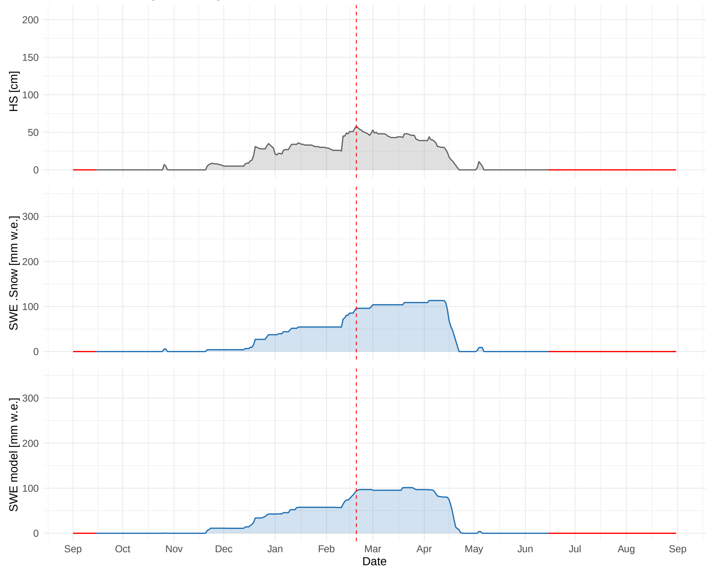
HSD_CH_SAM_MAN (1708 m a.s.l.) – 1986 to 1987
