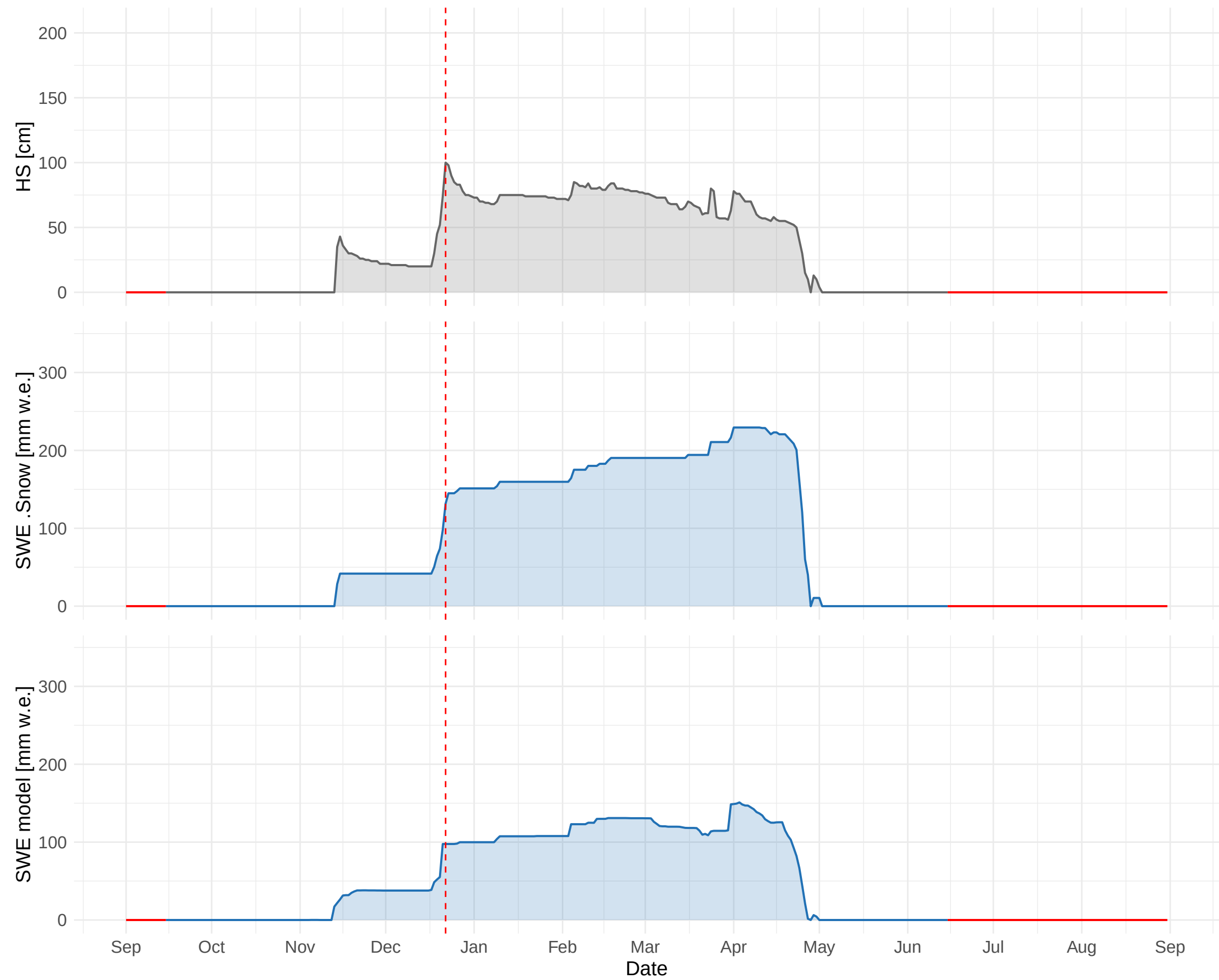
HSD_CH_SAM_MAN (1708 m a.s.l.) – 1991 to 1992
