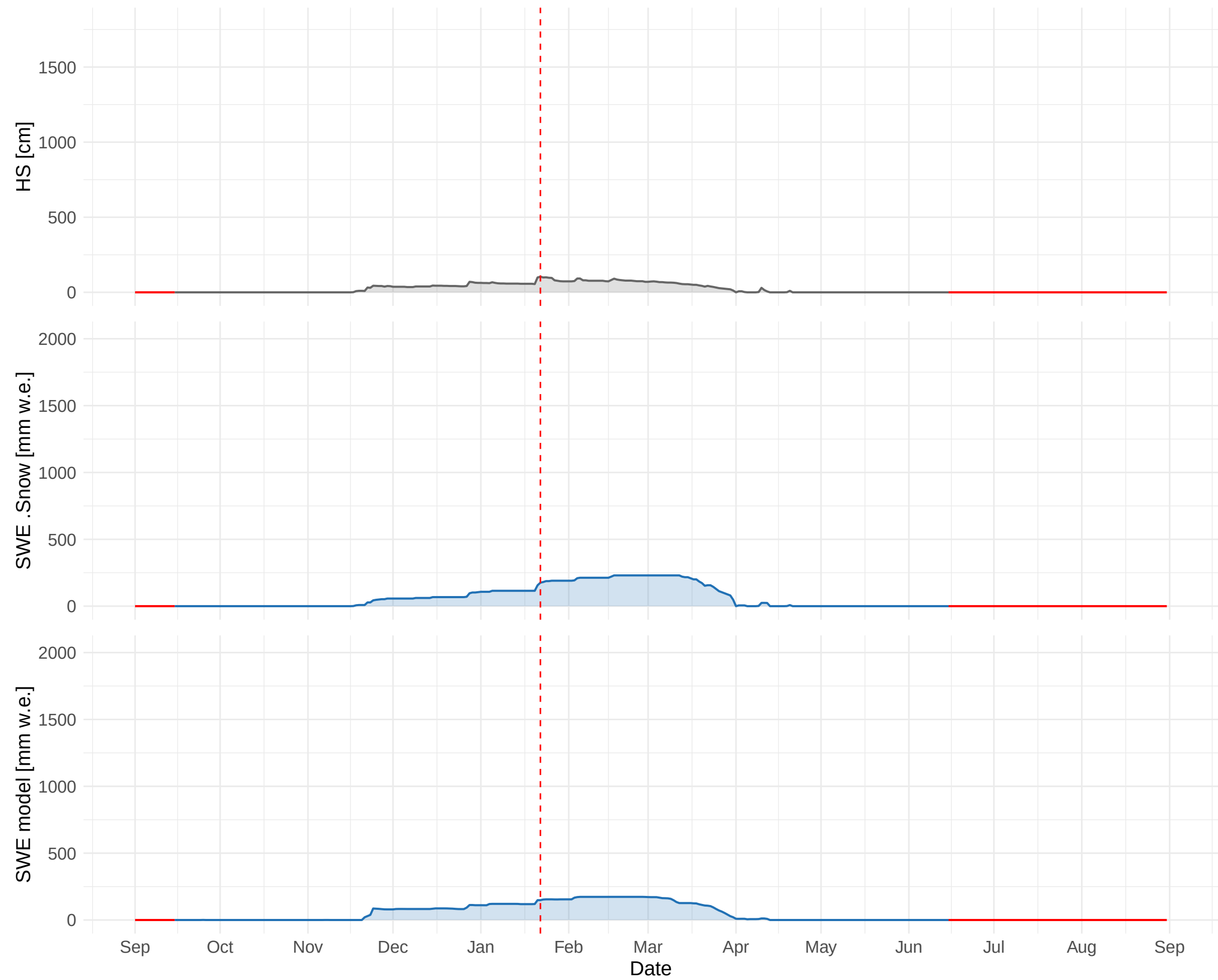
HSD_CH_SBE_MAN (1638 m a.s.l.) – 2002 to 2003
