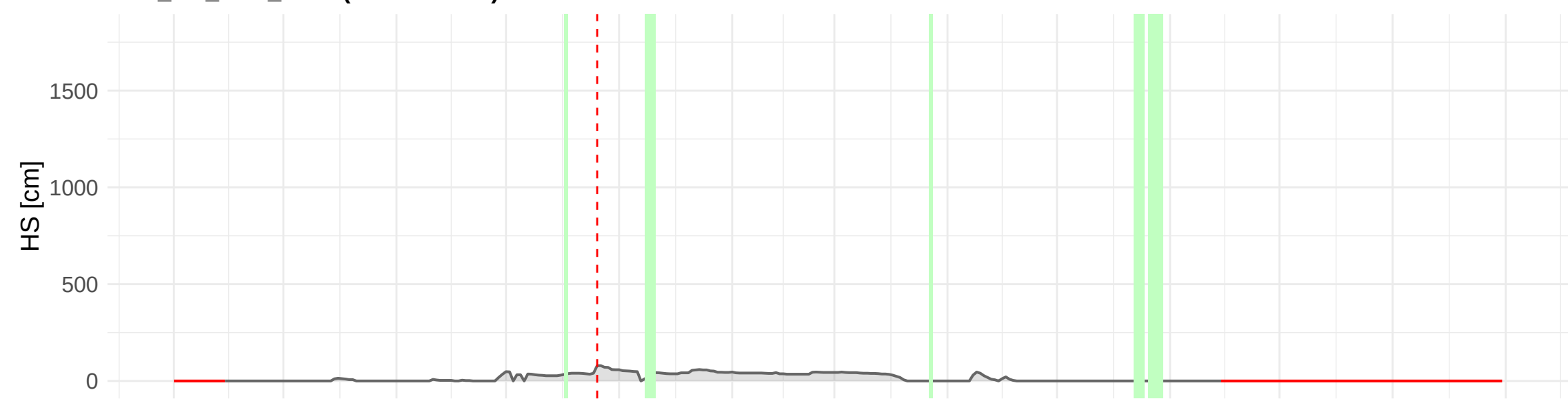
HSD_CH_SBE_MAN (1638 m a.s.l.) – 2004 to 2005
