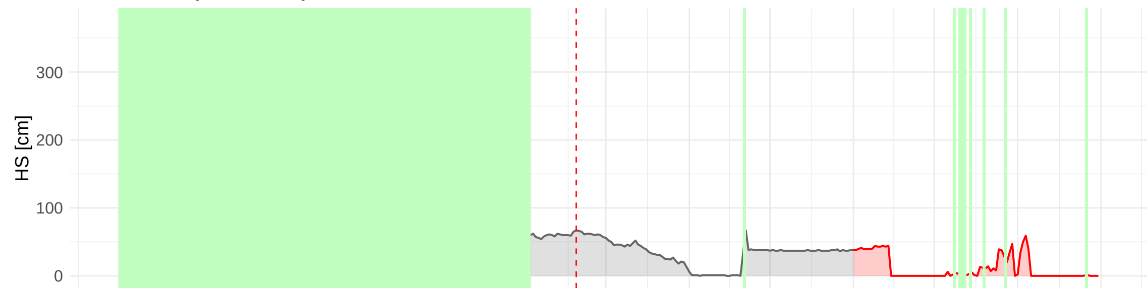
HSD_CH_SCU (1303 m a.s.l.) – 2008 to 2009
