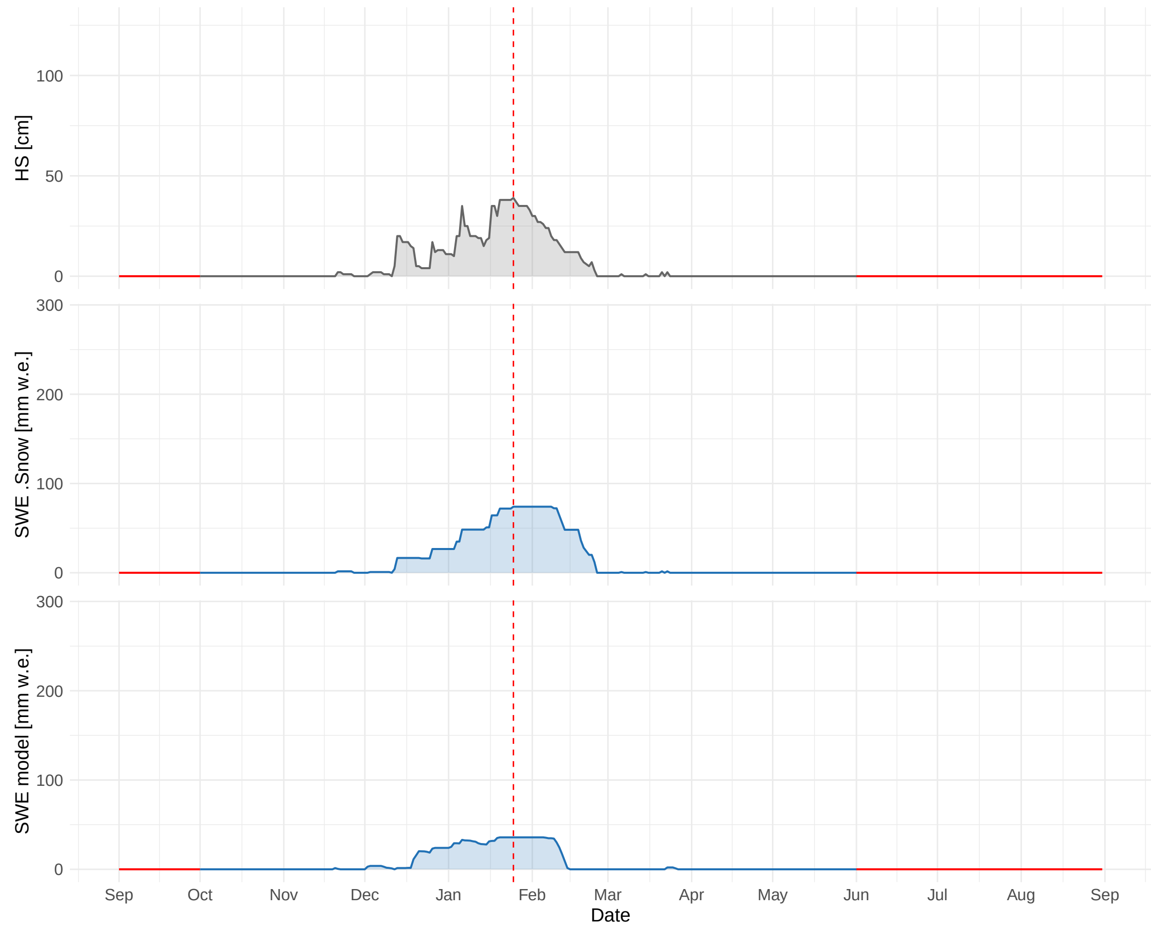
HSD_CH_SCU_MAN (1303 m a.s.l.) – 1997 to 1998
