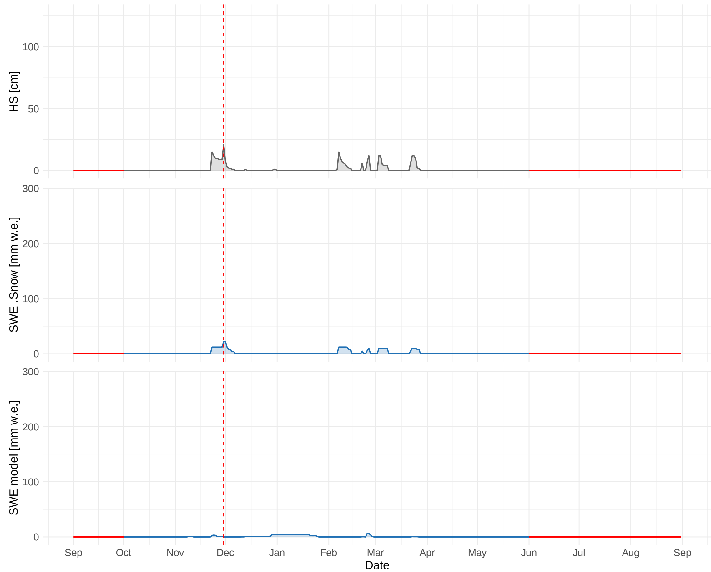
HSD_CH_SCU_MAN (1303 m a.s.l.) – 2001 to 2002
