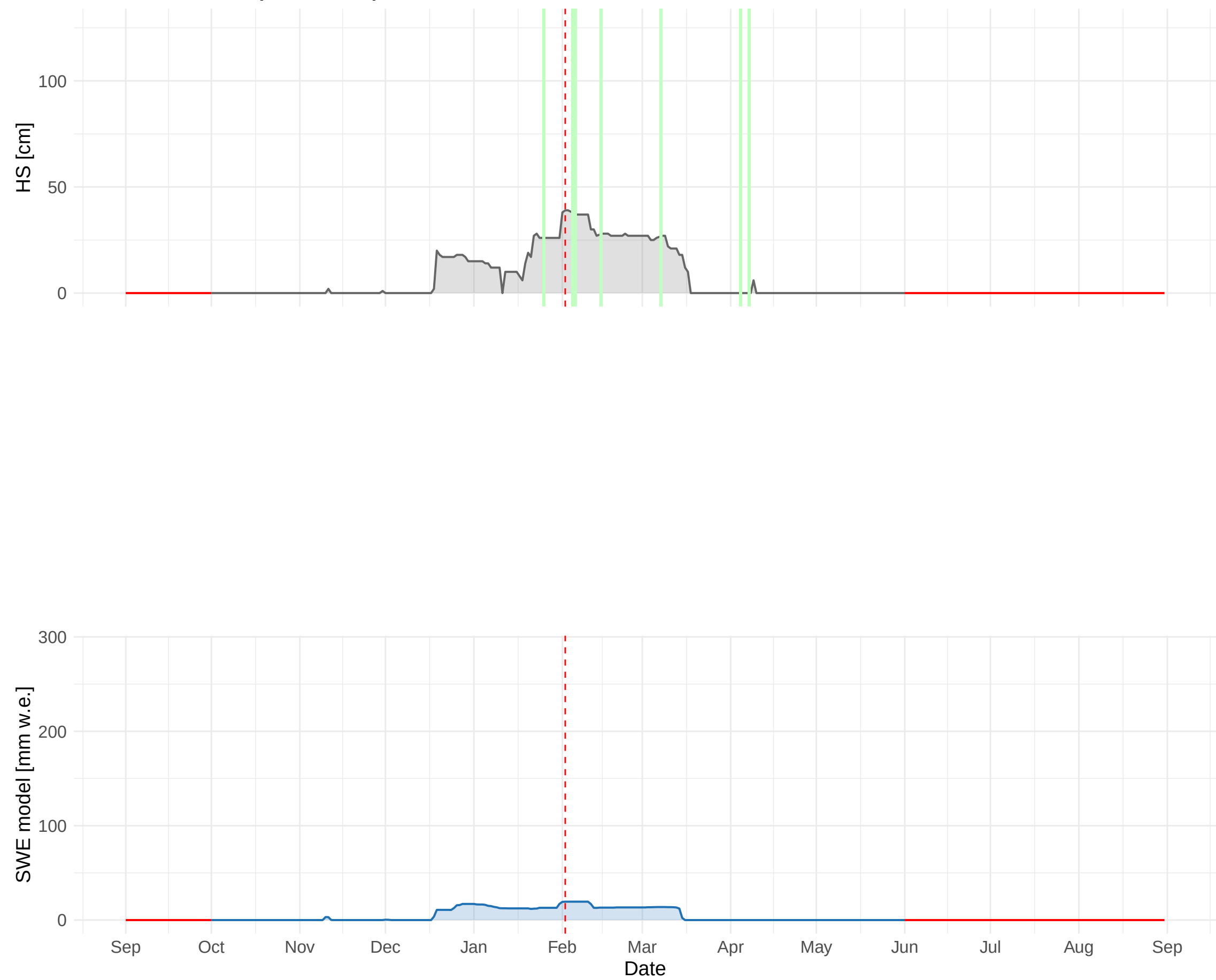
HSD_CH_SCU_MAN (1303 m a.s.l.) – 2004 to 2005
