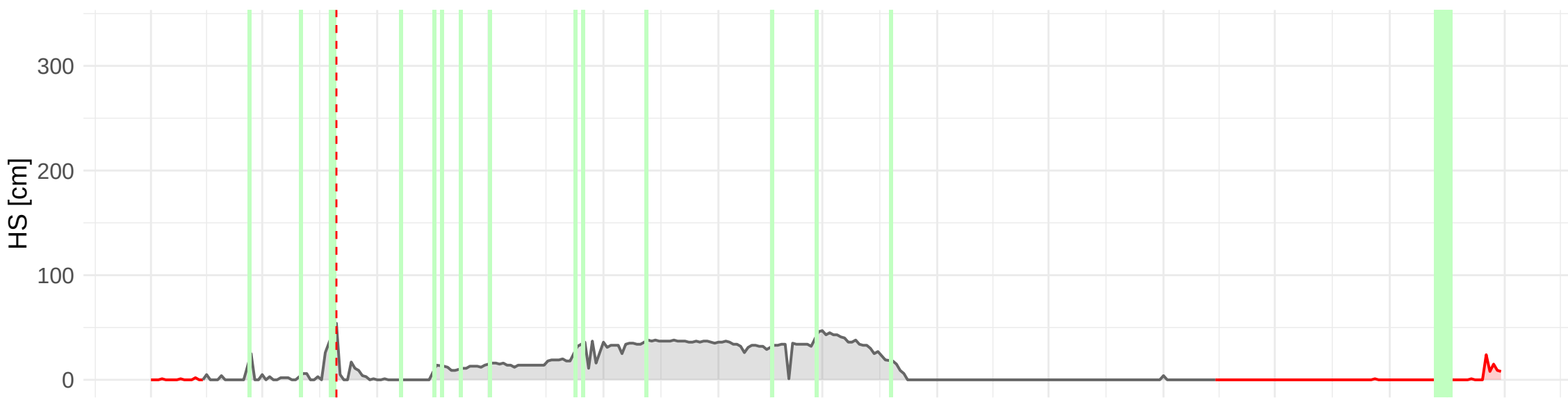
HSD_CH_ZER (1638 m a.s.l.) – 2010 to 2011
